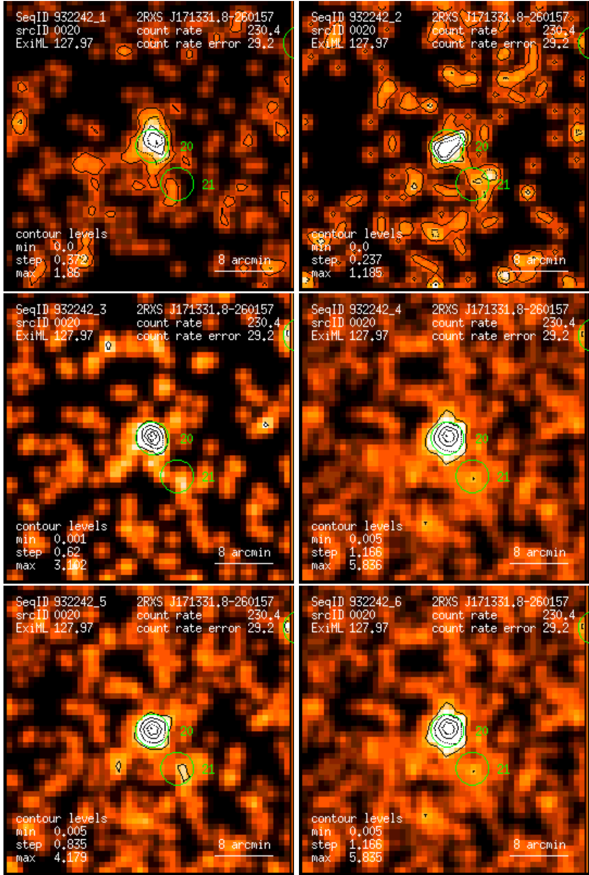
Figure 20: RASS 932242: detection 0020: band rate images, Gaussian filter: (1) PSPC channels 11 – 41, (2) 52 – 90, (3) 91 – 201, (4) 11 – 235, (5) 52 – 201, (6) 11 – 201. Broad band rates in counts/ks. Band rate contour levels in counts/ks/arcmin 2 .
