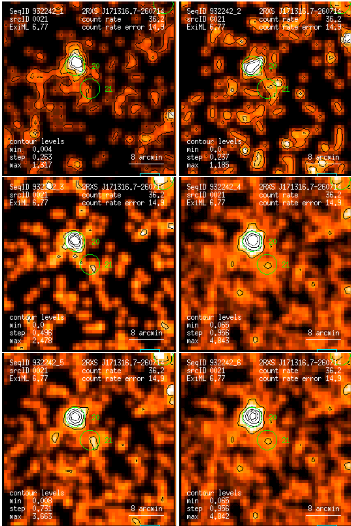
Figure 21: RASS 932242: detection 0021: band rate images, Gaussian filter: (1) PSPC channels 11 – 41, (2) 52 – 90, (3) 91 – 201, (4) 11 – 235, (5) 52 – 201, (6) 11 – 201. Broad band rates in counts/ks. Band rate contour levels in counts/ks/arcmin 2 .
