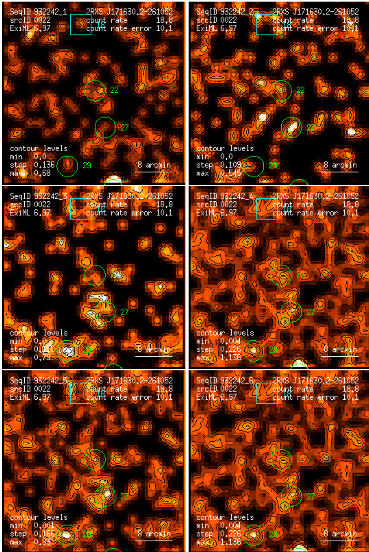
Figure 22: RASS 932242: detection 0022: band rate images, Gaussian filter: (1) PSPC channels 11 – 41, (2) 52 – 90, (3) 91 – 201, (4) 11 – 235, (5) 52 – 201, (6) 11 – 201. Broad band rates in counts/ks. Band rate contour levels in counts/ks/arcmin 2 .
