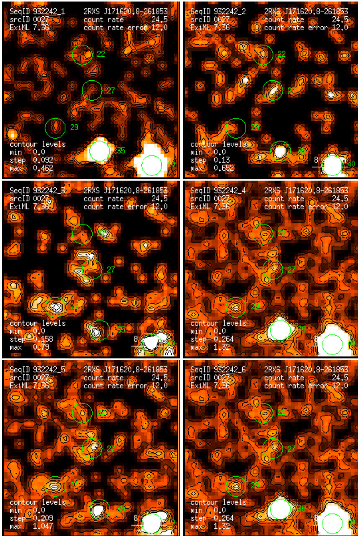
Figure 27: RASS 932242: detection 0027: band rate images, Gaussian filter: (1) PSPC channels 11 – 41, (2) 52 – 90, (3) 91 – 201, (4) 11 – 235, (5) 52 – 201, (6) 11 – 201. Broad band rates in counts/ks. Band rate contour levels in counts/ks/arcmin 2 .
