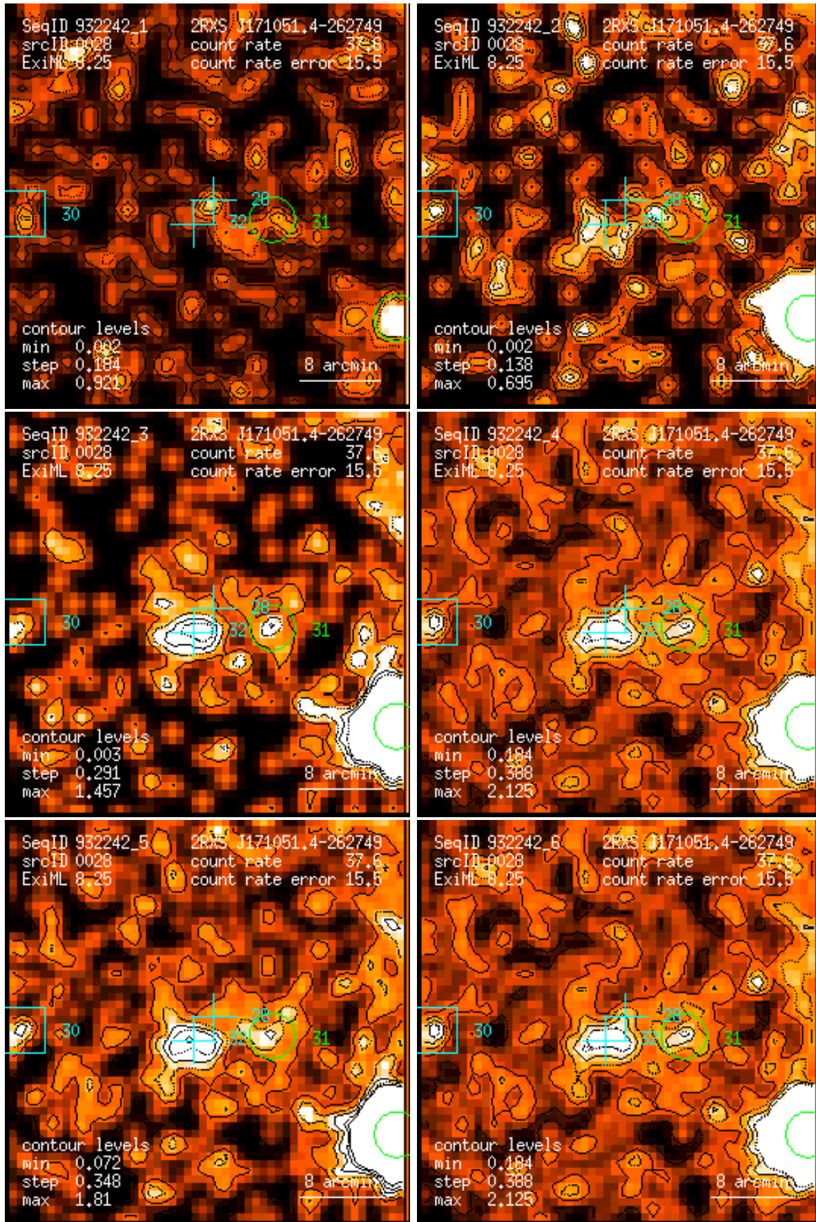
Figure 28: RASS 932242: detection 0028: band rate images, Gaussian filter: (1) PSPC channels 11 – 41, (2) 52 – 90, (3) 91 – 201, (4) 11 – 235, (5) 52 – 201, (6) 11 – 201. Broad band rates in counts/ks. Band rate contour levels in counts/ks/arcmin 2 .
