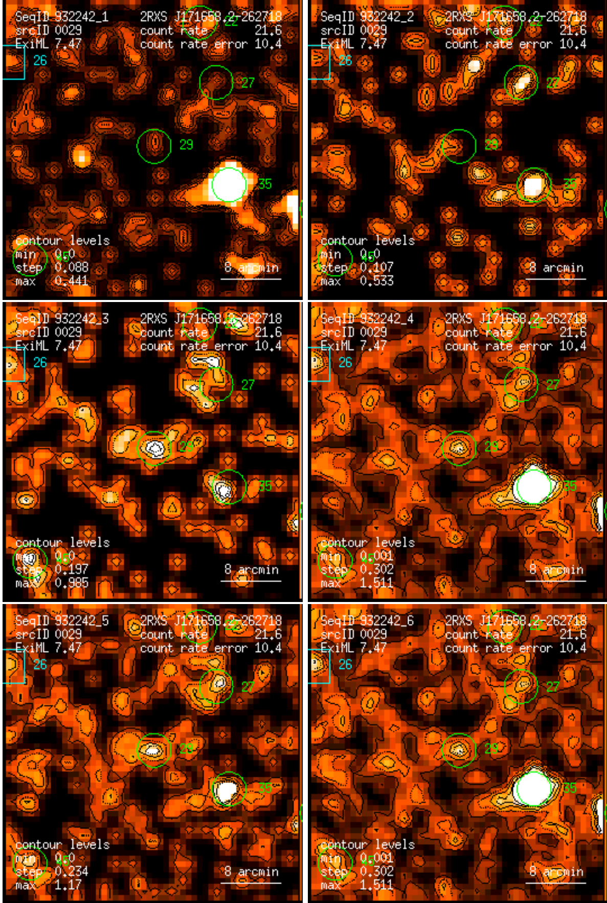
Figure 29: RASS 932242: detection 0029: band rate images, Gaussian filter: (1) PSPC channels 11 – 41, (2) 52 – 90, (3) 91 – 201, (4) 11 – 235, (5) 52 – 201, (6) 11 – 201. Broad band rates in counts/ks. Band rate contour levels in counts/ks/arcmin 2 .
