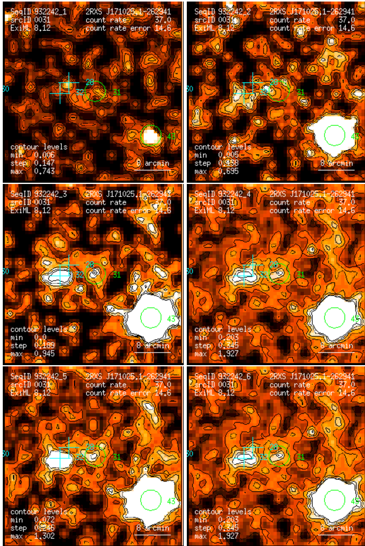
Figure 31: RASS 932242: detection 0031: band rate images, Gaussian filter: (1) PSPC channels 11 – 41, (2) 52 – 90, (3) 91 – 201, (4) 11 – 235, (5) 52 – 201, (6) 11 – 201. Broad band rates in counts/ks. Band rate contour levels in counts/ks/arcmin 2 .
