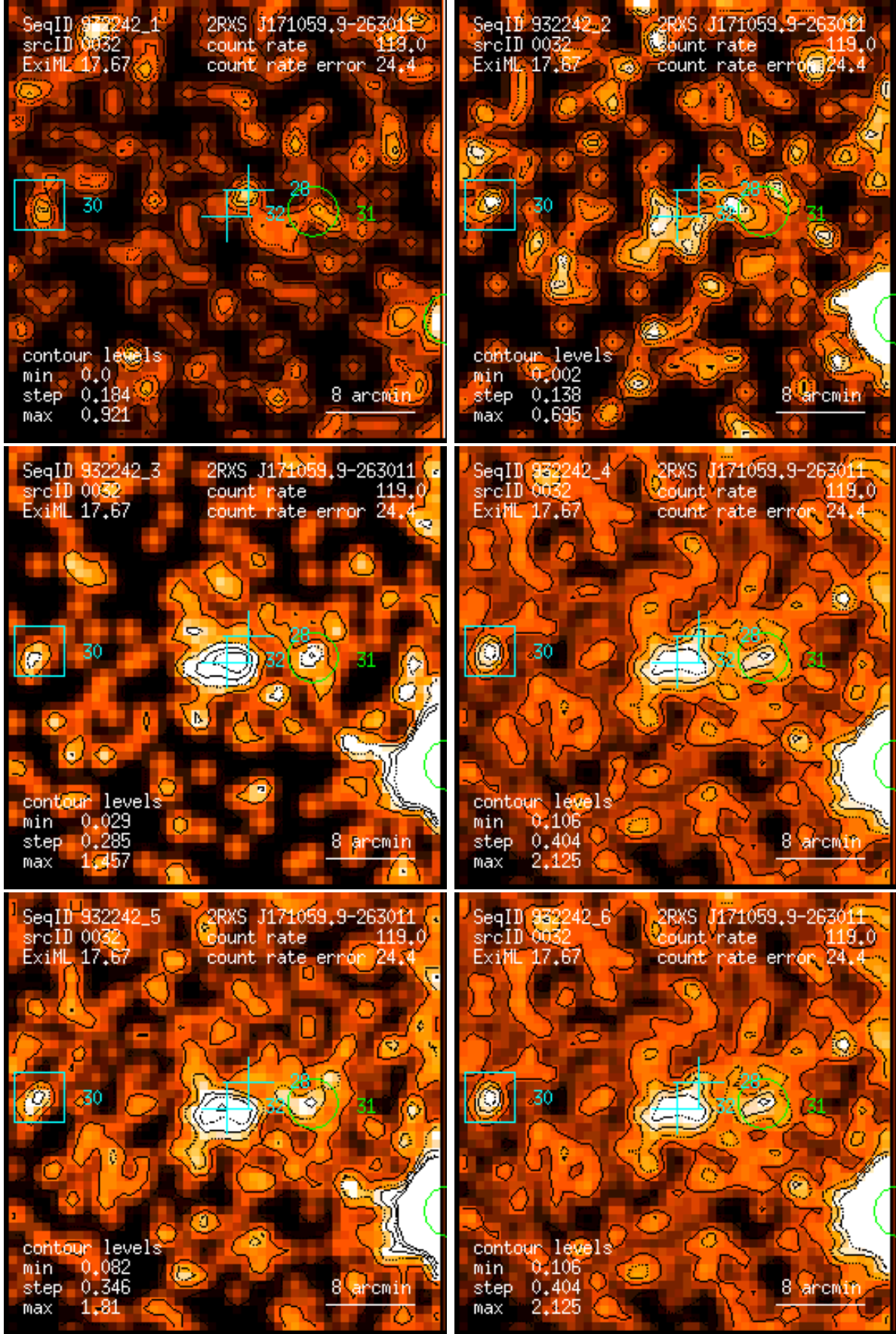
Figure 32: RASS 932242: detection 0032: band rate images, Gaussian filter: (1) PSPC channels 11 – 41, (2) 52 – 90, (3) 91 – 201, (4) 11 – 235, (5) 52 – 201, (6) 11 – 201. Broad band rates in counts/ks. Band rate contour levels in counts/ks/arcmin 2 .
