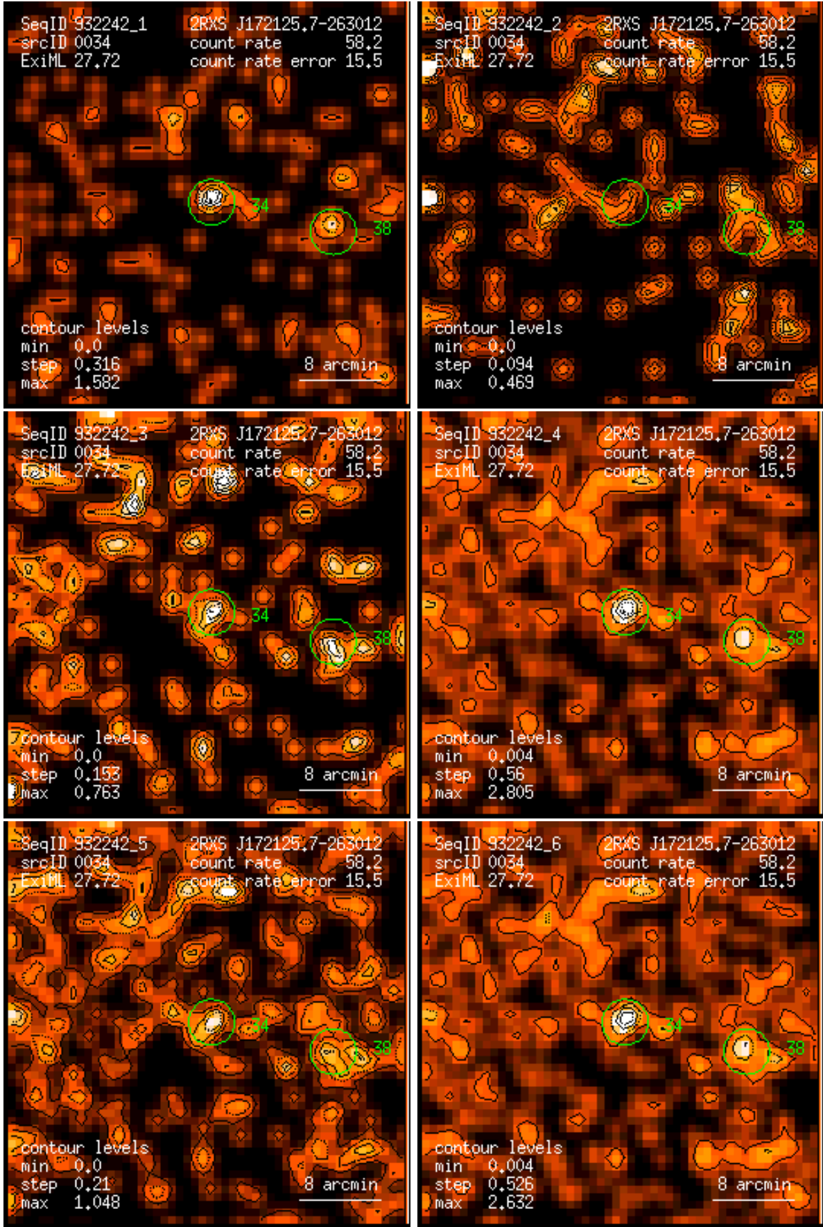
Figure 34: RASS 932242: detection 0034: band rate images, Gaussian filter: (1) PSPC channels 11 – 41, (2) 52 – 90, (3) 91 – 201, (4) 11 – 235, (5) 52 – 201, (6) 11 – 201. Broad band rates in counts/ks. Band rate contour levels in counts/ks/arcmin 2 .
