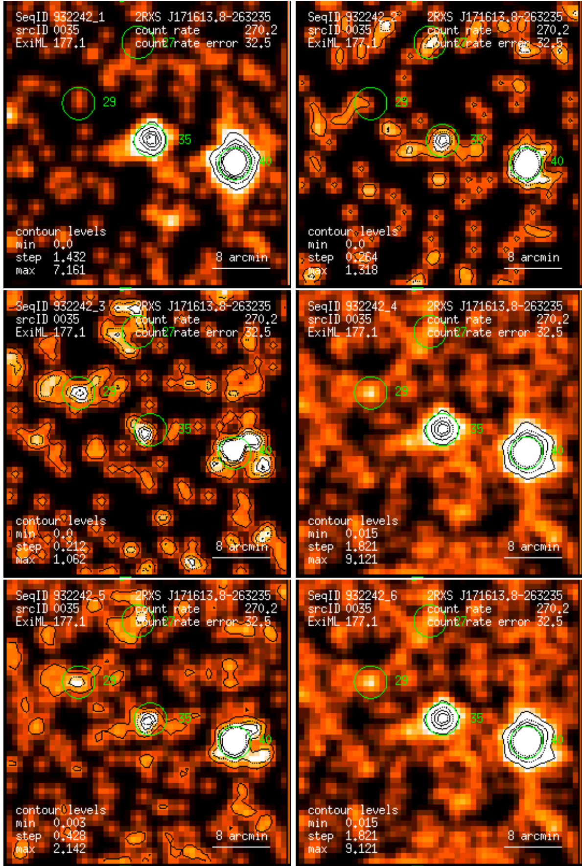
Figure 35: RASS 932242: detection 0035: band rate images, Gaussian filter: (1) PSPC channels 11 – 41, (2) 52 – 90, (3) 91 – 201, (4) 11 – 235, (5) 52 – 201, (6) 11 – 201. Broad band rates in counts/ks. Band rate contour levels in counts/ks/arcmin 2 .
