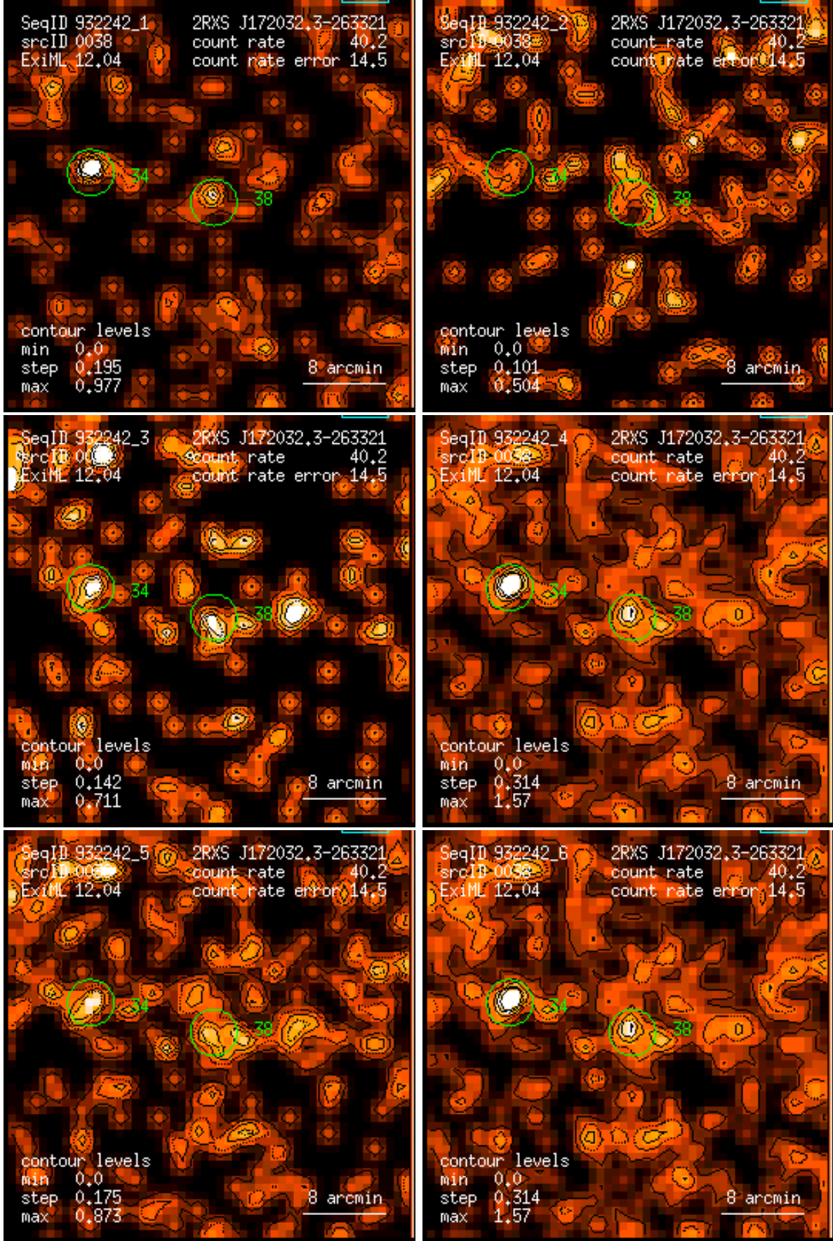
Figure 38: RASS 932242: detection 0038: band rate images, Gaussian filter: (1) PSPC channels 11 – 41, (2) 52 – 90, (3) 91 – 201, (4) 11 – 235, (5) 52 – 201, (6) 11 – 201. Broad band rates in counts/ks. Band rate contour levels in counts/ks/arcmin 2 .
