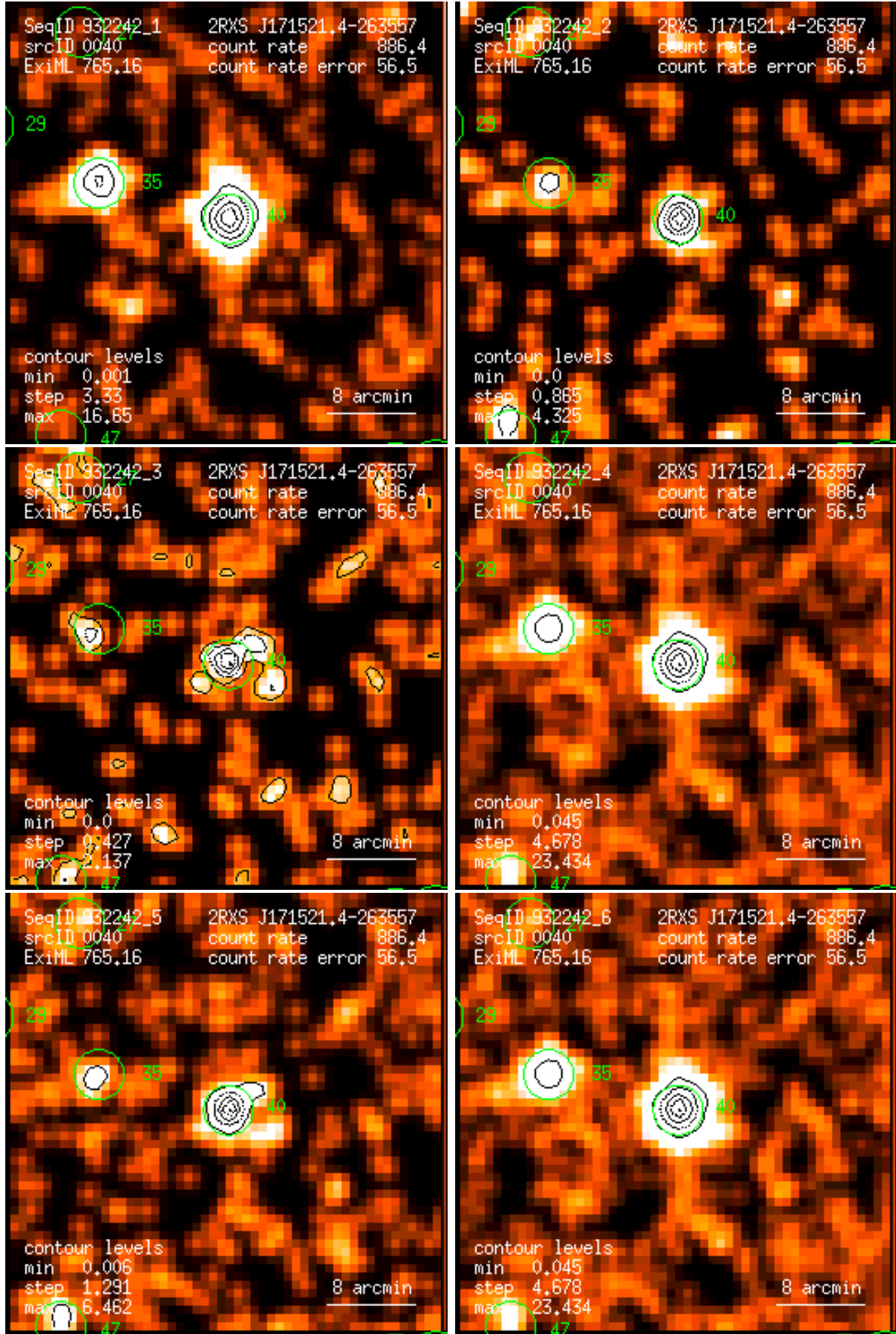
Figure 40: RASS 932242: detection 0040: band rate images, Gaussian filter: (1) PSPC channels 11 – 41, (2) 52 – 90, (3) 91 – 201, (4) 11 – 235, (5) 52 – 201, (6) 11 – 201. Broad band rates in counts/ks. Band rate contour levels in counts/ks/arcmin 2 .
