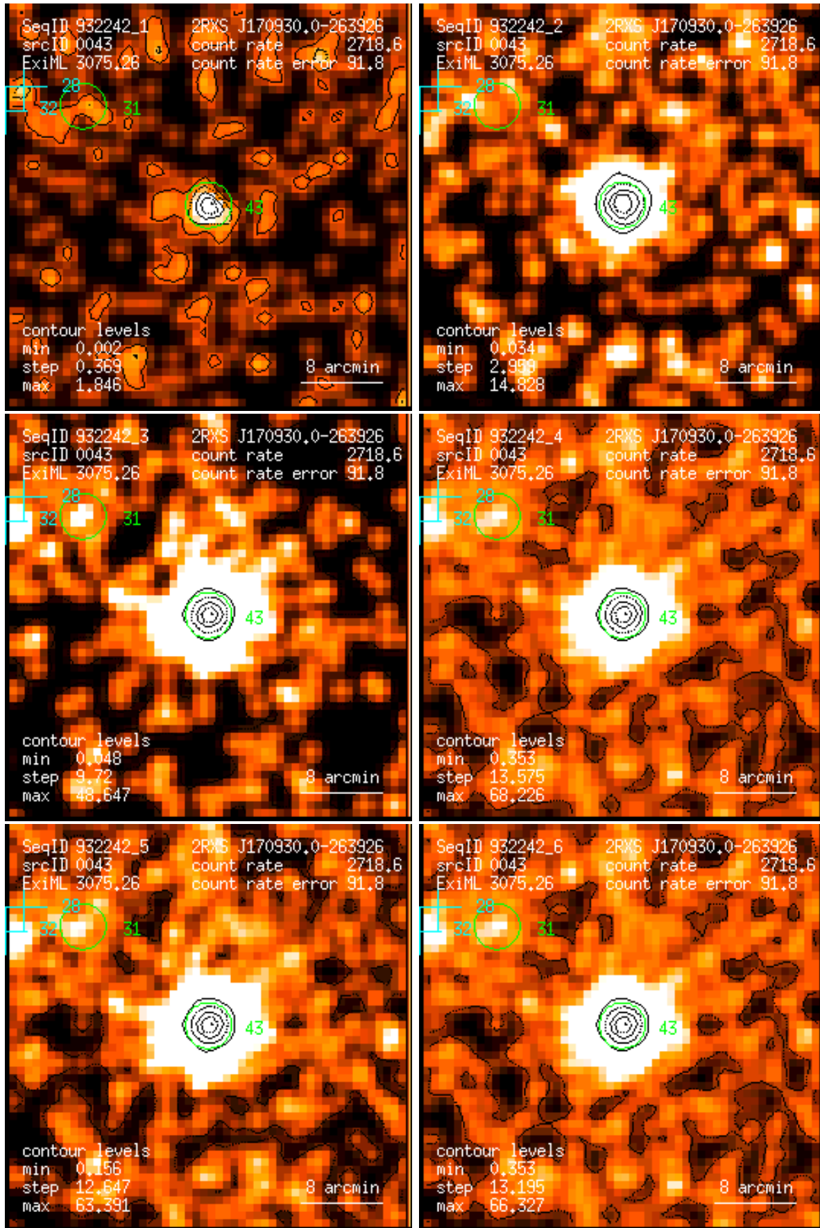
Figure 43: RASS 932242: detection 0043: band rate images, Gaussian filter: (1) PSPC channels 11 – 41, (2) 52 – 90, (3) 91 – 201, (4) 11 – 235, (5) 52 – 201, (6) 11 – 201. Broad band rates in counts/ks. Band rate contour levels in counts/ks/arcmin 2 .
