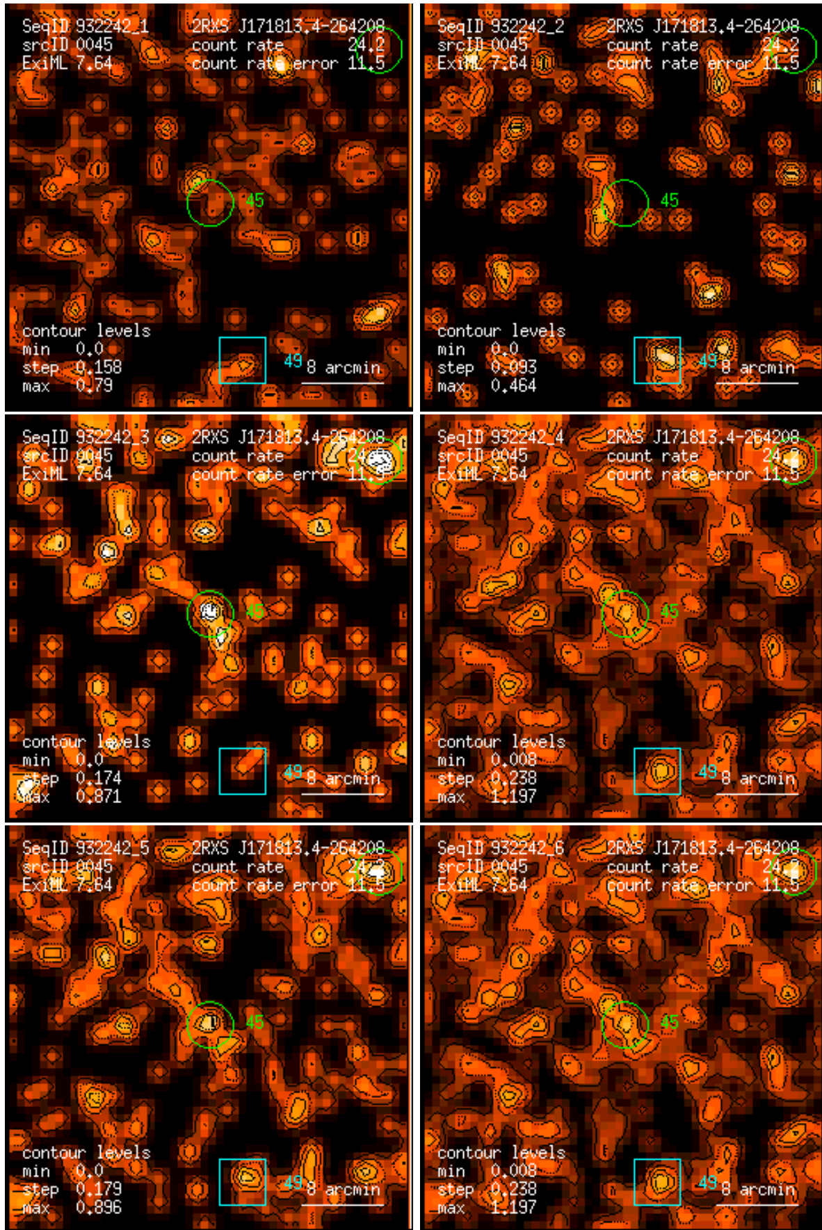
Figure 45: RASS 932242: detection 0045: band rate images, Gaussian filter: (1) PSPC channels 11 – 41, (2) 52 – 90, (3) 91 – 201, (4) 11 – 235, (5) 52 – 201, (6) 11 – 201. Broad band rates in counts/ks. Band rate contour levels in counts/ks/arcmin 2 .
