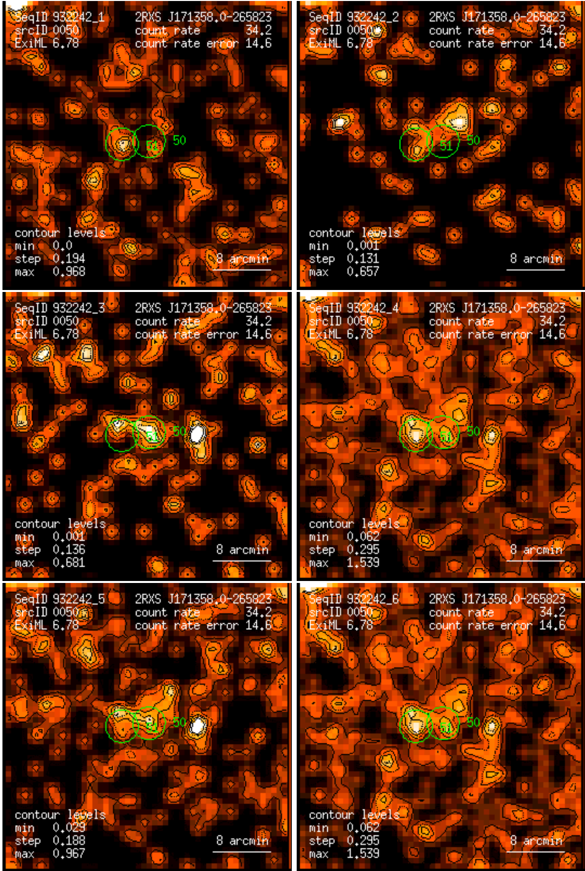
Figure 50: RASS 932242: detection 0050: band rate images, Gaussian filter: (1) PSPC channels 11 – 41, (2) 52 – 90, (3) 91 – 201, (4) 11 – 235, (5) 52 – 201, (6) 11 – 201. Broad band rates in counts/ks. Band rate contour levels in counts/ks/arcmin 2 .
