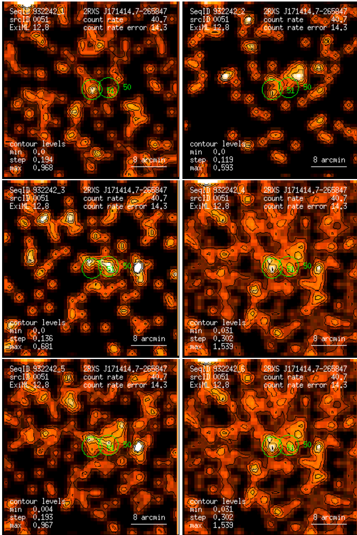
Figure 51: RASS 932242: detection 0051: band rate images, Gaussian filter: (1) PSPC channels 11 – 41, (2) 52 – 90, (3) 91 – 201, (4) 11 – 235, (5) 52 – 201, (6) 11 – 201. Broad band rates in counts/ks. Band rate contour levels in counts/ks/arcmin 2 .
