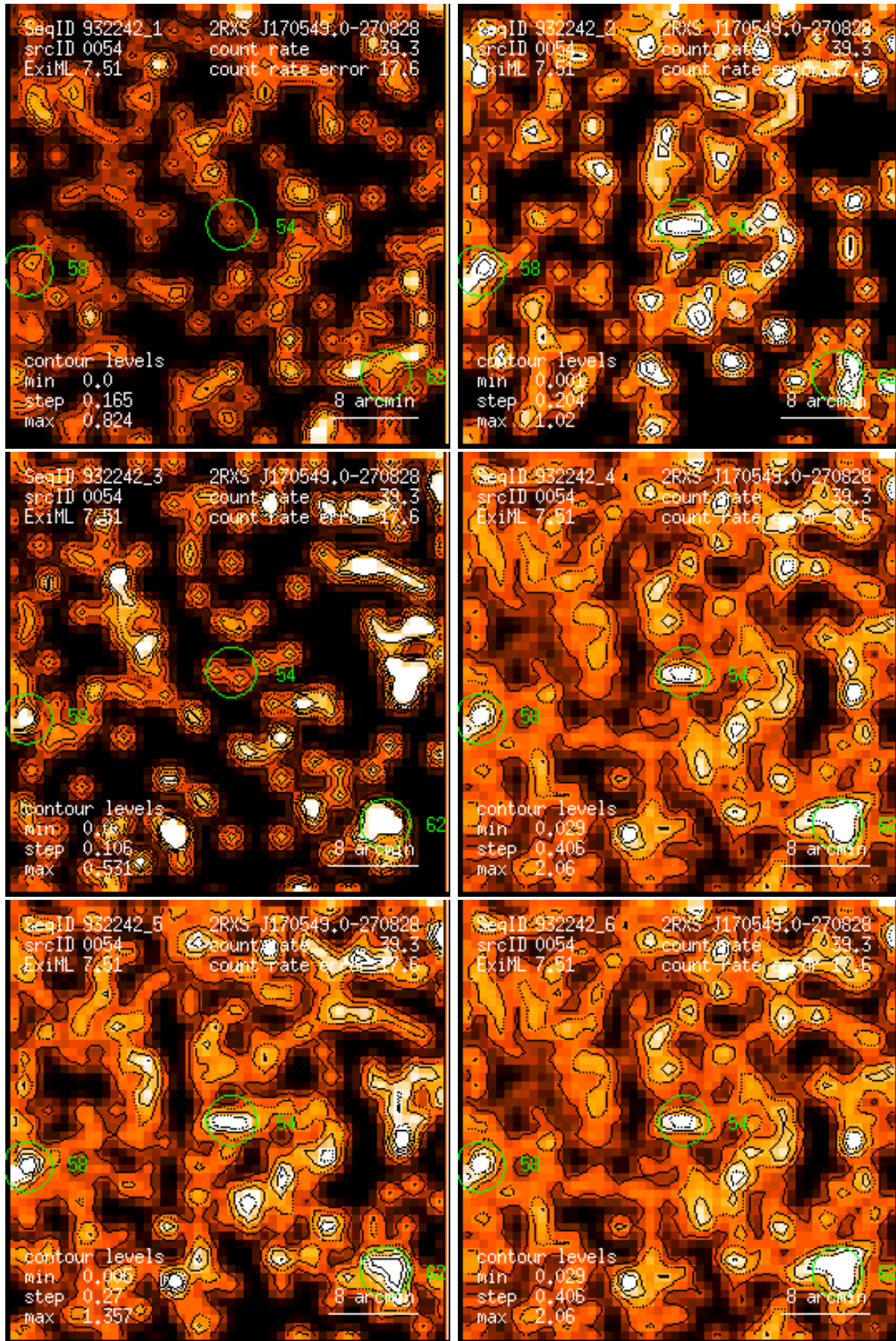
Figure 54: RASS 932242: detection 0054: band rate images, Gaussian filter: (1) PSPC channels 11 – 41, (2) 52 – 90, (3) 91 – 201, (4) 11 – 235, (5) 52 – 201, (6) 11 – 201. Broad band rates in counts/ks. Band rate contour levels in counts/ks/arcmin 2 .
