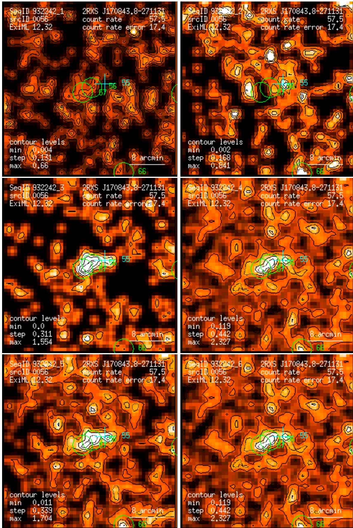
Figure 56: RASS 932242: detection 0056: band rate images, Gaussian filter: (1) PSPC channels 11 – 41, (2) 52 – 90, (3) 91 – 201, (4) 11 – 235, (5) 52 – 201, (6) 11 – 201. Broad band rates in counts/ks. Band rate contour levels in counts/ks/arcmin 2 .
