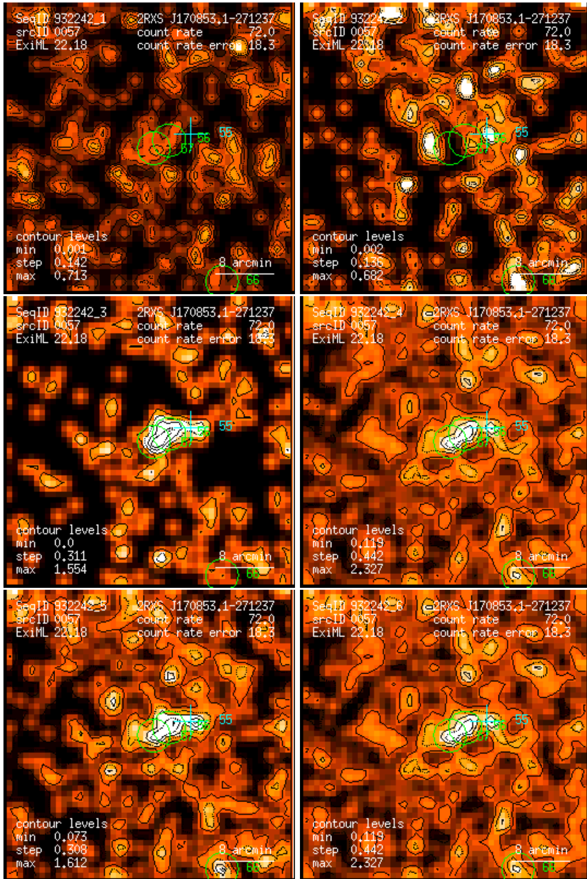
Figure 57: RASS 932242: detection 0057: band rate images, Gaussian filter: (1) PSPC channels 11 – 41, (2) 52 – 90, (3) 91 – 201, (4) 11 – 235, (5) 52 – 201, (6) 11 – 201. Broad band rates in counts/ks. Band rate contour levels in counts/ks/arcmin 2 .
