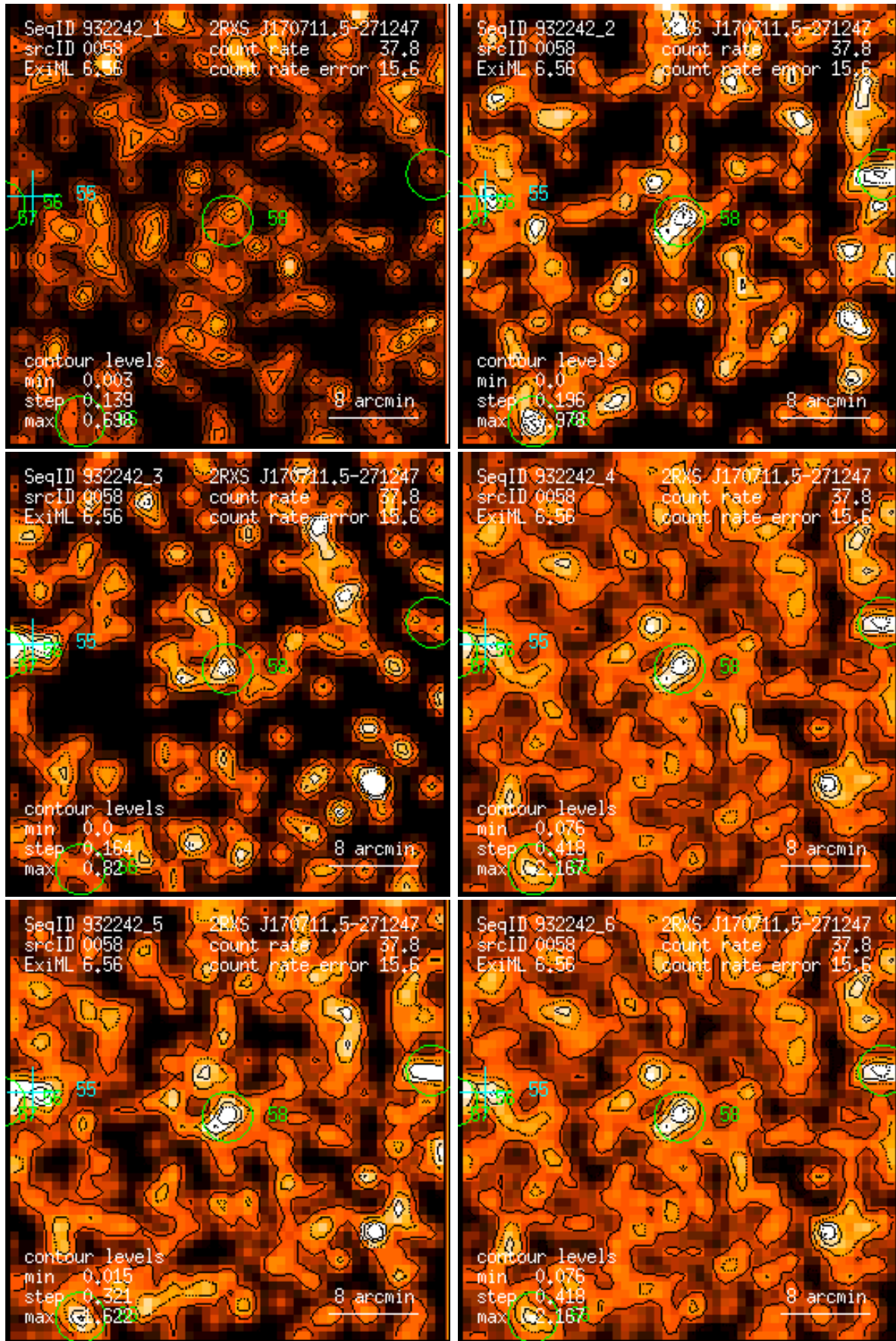
Figure 58: RASS 932242: detection 0058: band rate images, Gaussian filter: (1) PSPC channels 11 – 41, (2) 52 – 90, (3) 91 – 201, (4) 11 – 235, (5) 52 – 201, (6) 11 – 201. Broad band rates in counts/ks. Band rate contour levels in counts/ks/arcmin 2 .
