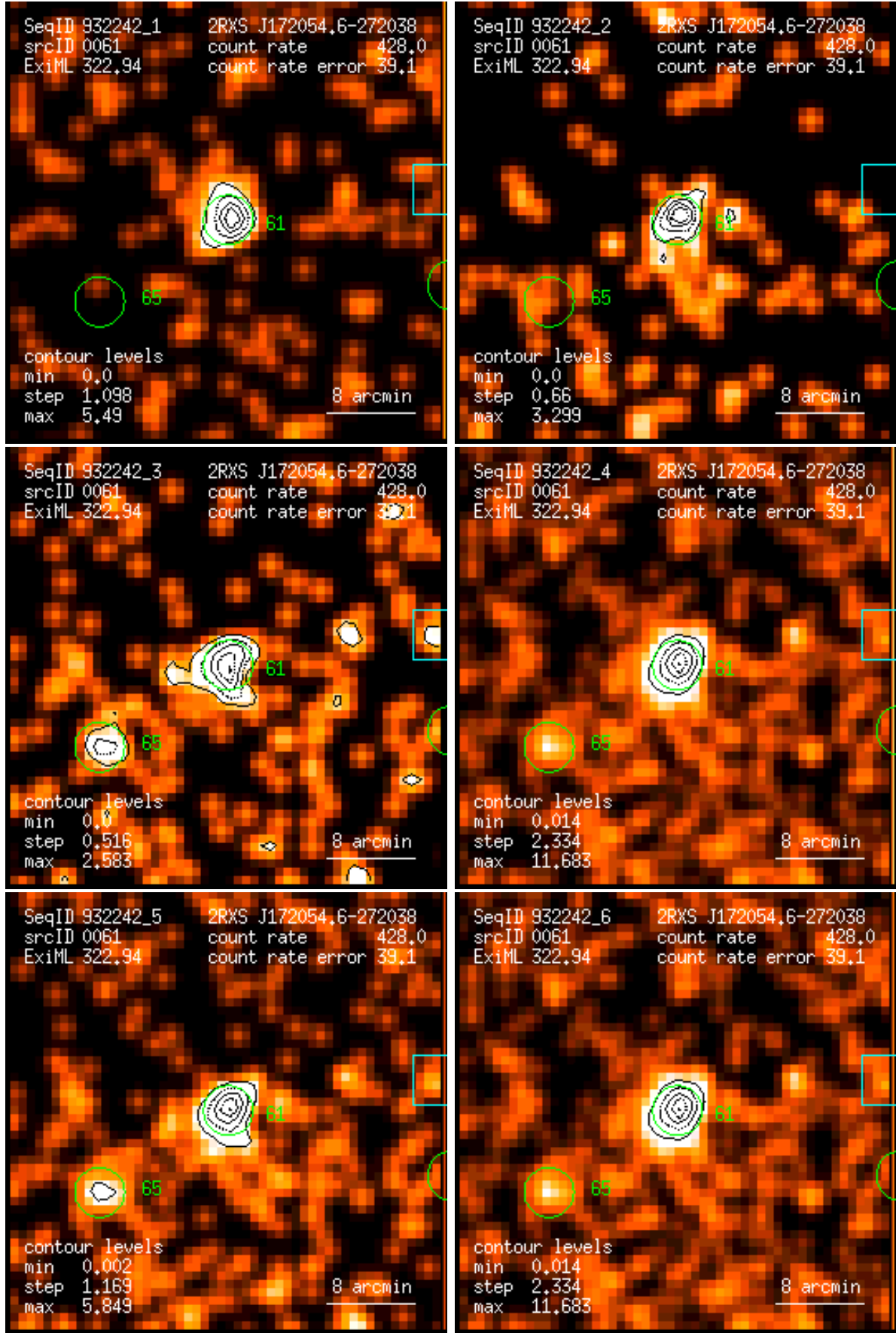
Figure 61: RASS 932242: detection 0061: band rate images, Gaussian filter: (1) PSPC channels 11 – 41, (2) 52 – 90, (3) 91 – 201, (4) 11 – 235, (5) 52 – 201, (6) 11 – 201. Broad band rates in counts/ks. Band rate contour levels in counts/ks/arcmin 2 .
