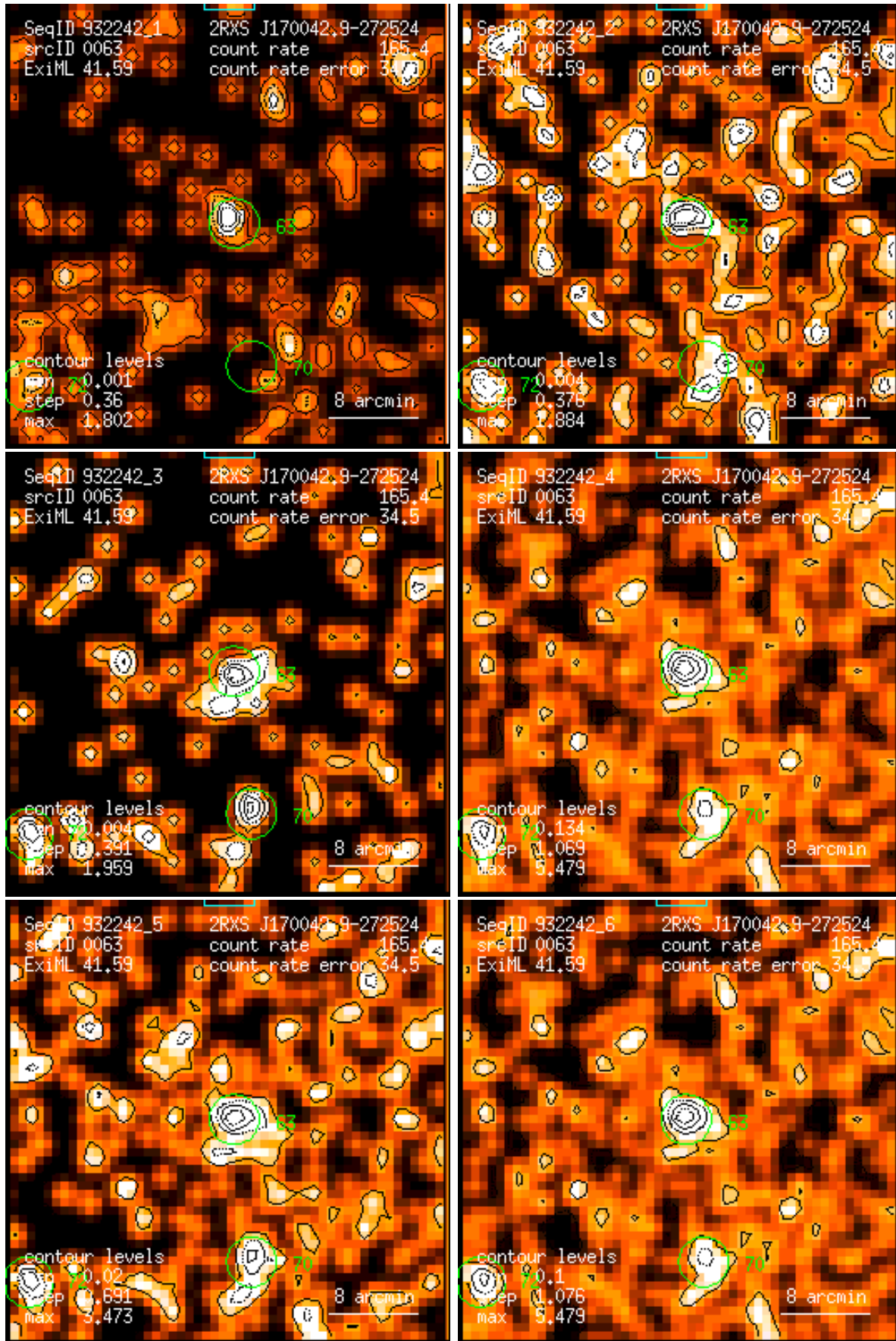
Figure 63: RASS 932242: detection 0063: band rate images, Gaussian filter: (1) PSPC channels 11 – 41, (2) 52 – 90, (3) 91 – 201, (4) 11 – 235, (5) 52 – 201, (6) 11 – 201. Broad band rates in counts/ks. Band rate contour levels in counts/ks/arcmin 2 .
