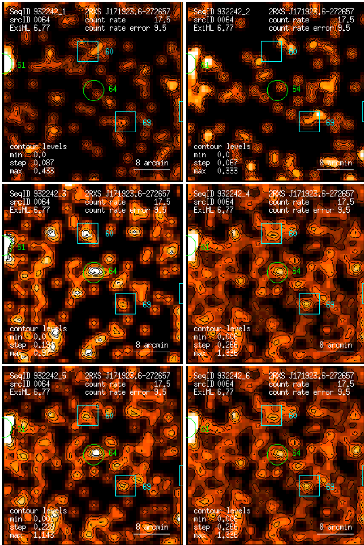
Figure 64: RASS 932242: detection 0064: band rate images, Gaussian filter: (1) PSPC channels 11 – 41, (2) 52 – 90, (3) 91 – 201, (4) 11 – 235, (5) 52 – 201, (6) 11 – 201. Broad band rates in counts/ks. Band rate contour levels in counts/ks/arcmin 2 .
