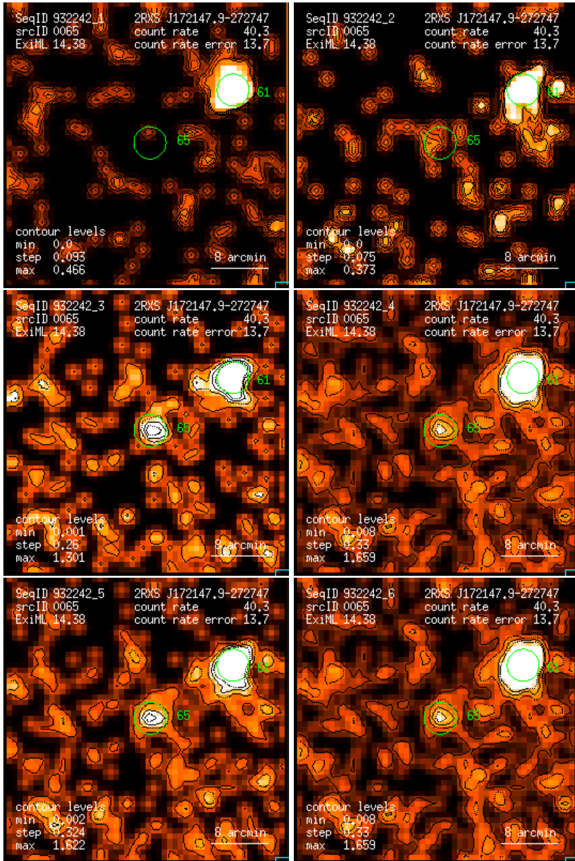
Figure 65: RASS 932242: detection 0065: band rate images, Gaussian filter: (1) PSPC channels 11 – 41, (2) 52 – 90, (3) 91 – 201, (4) 11 – 235, (5) 52 – 201, (6) 11 – 201. Broad band rates in counts/ks. Band rate contour levels in counts/ks/arcmin 2 .
