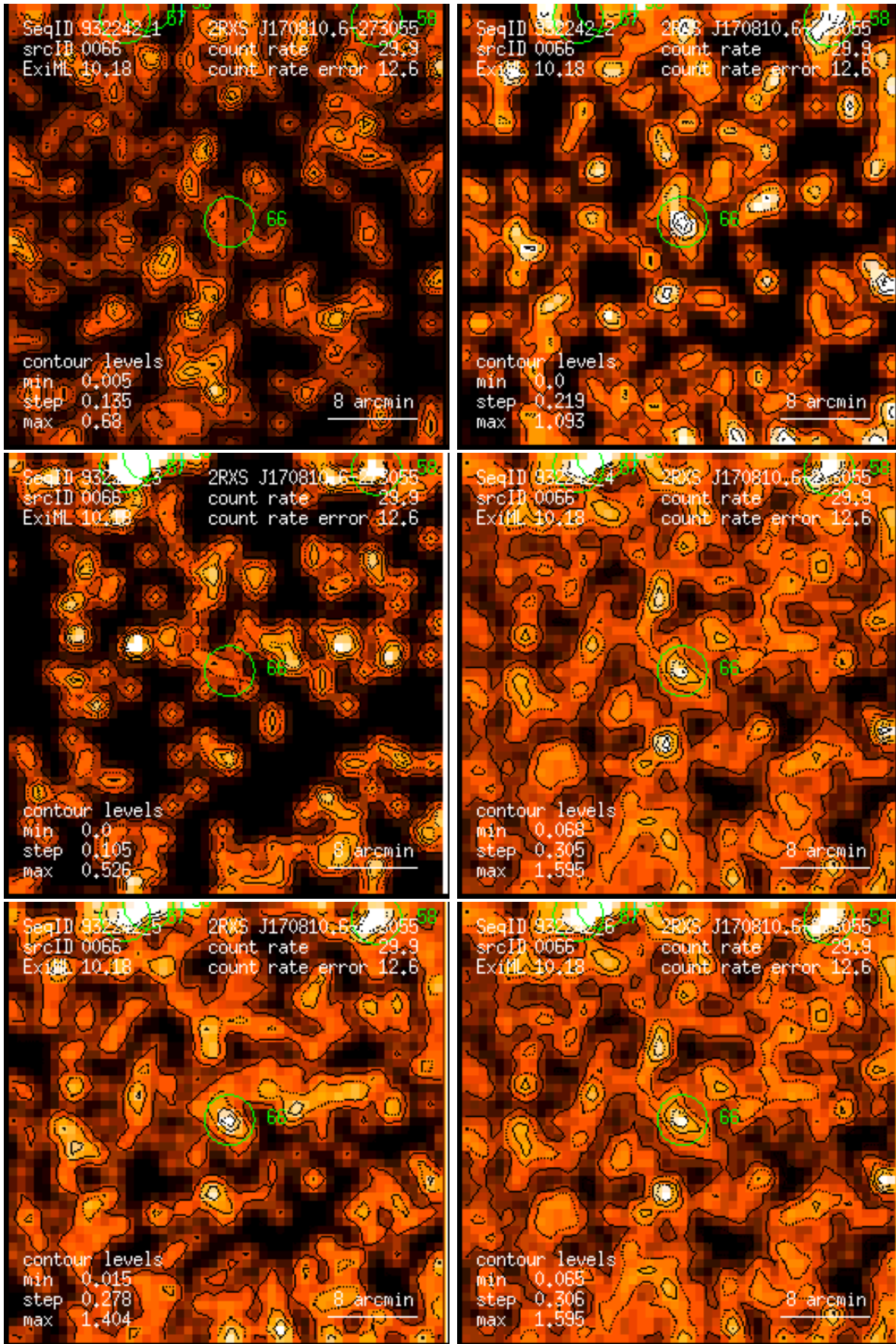
Figure 66: RASS 932242: detection 0066: band rate images, Gaussian filter: (1) PSPC channels 11 – 41, (2) 52 – 90, (3) 91 – 201, (4) 11 – 235, (5) 52 – 201, (6) 11 – 201. Broad band rates in counts/ks. Band rate contour levels in counts/ks/arcmin 2 .
