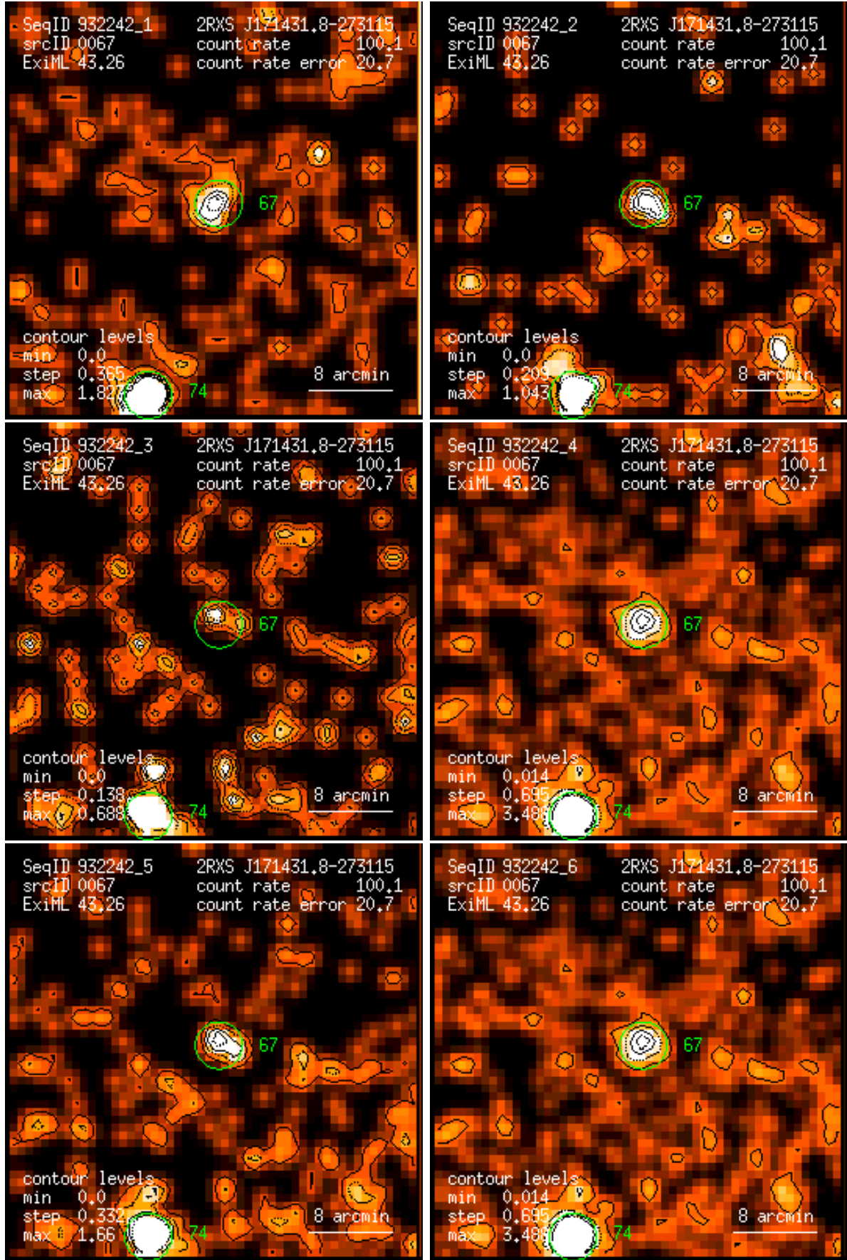
Figure 67: RASS 932242: detection 0067: band rate images, Gaussian filter: (1) PSPC channels 11 – 41, (2) 52 – 90, (3) 91 – 201, (4) 11 – 235, (5) 52 – 201, (6) 11 – 201. Broad band rates in counts/ks. Band rate contour levels in counts/ks/arcmin 2 .
