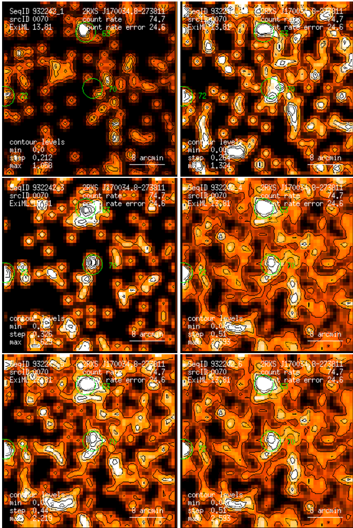
Figure 70: RASS 932242: detection 0070: band rate images, Gaussian filter: (1) PSPC channels 11 – 41, (2) 52 – 90, (3) 91 – 201, (4) 11 – 235, (5) 52 – 201, (6) 11 – 201. Broad band rates in counts/ks. Band rate contour levels in counts/ks/arcmin 2 .
