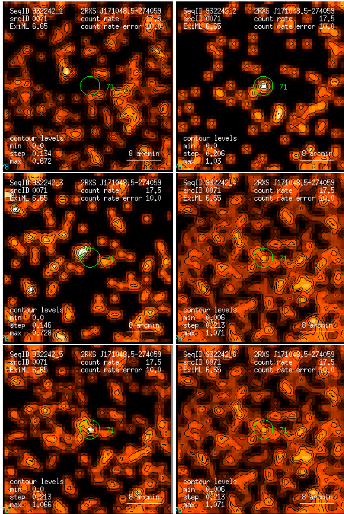
Figure 71: RASS 932242: detection 0071: band rate images, Gaussian filter: (1) PSPC channels 11 – 41, (2) 52 – 90, (3) 91 – 201, (4) 11 – 235, (5) 52 – 201, (6) 11 – 201. Broad band rates in counts/ks. Band rate contour levels in counts/ks/arcmin 2 .
