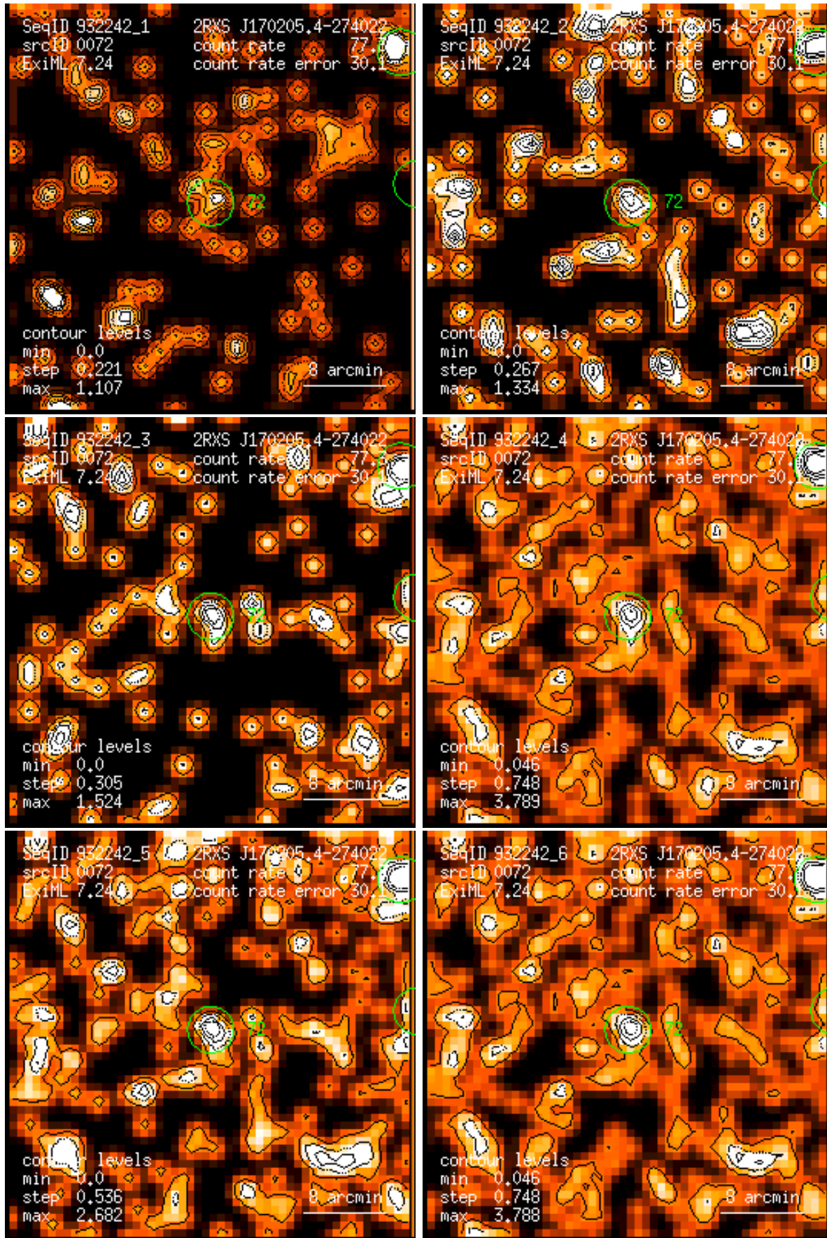
Figure 72: RASS 932242: detection 0072: band rate images, Gaussian filter: (1) PSPC channels 11 – 41, (2) 52 – 90, (3) 91 – 201, (4) 11 – 235, (5) 52 – 201, (6) 11 – 201. Broad band rates in counts/ks. Band rate contour levels in counts/ks/arcmin 2 .
