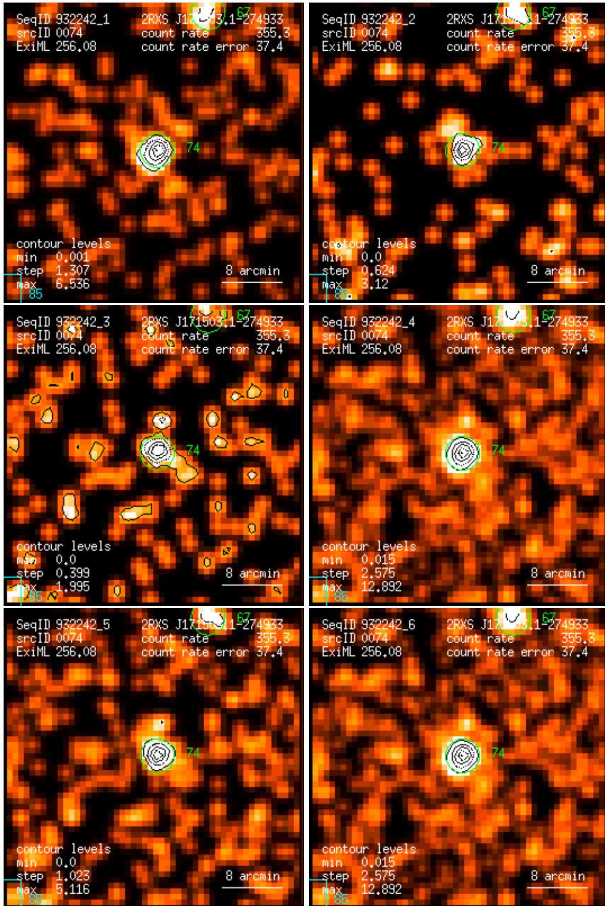
Figure 74: RASS 932242: detection 0074: band rate images, Gaussian filter: (1) PSPC channels 11 – 41, (2) 52 – 90, (3) 91 – 201, (4) 11 – 235, (5) 52 – 201, (6) 11 – 201. Broad band rates in counts/ks. Band rate contour levels in counts/ks/arcmin 2 .
