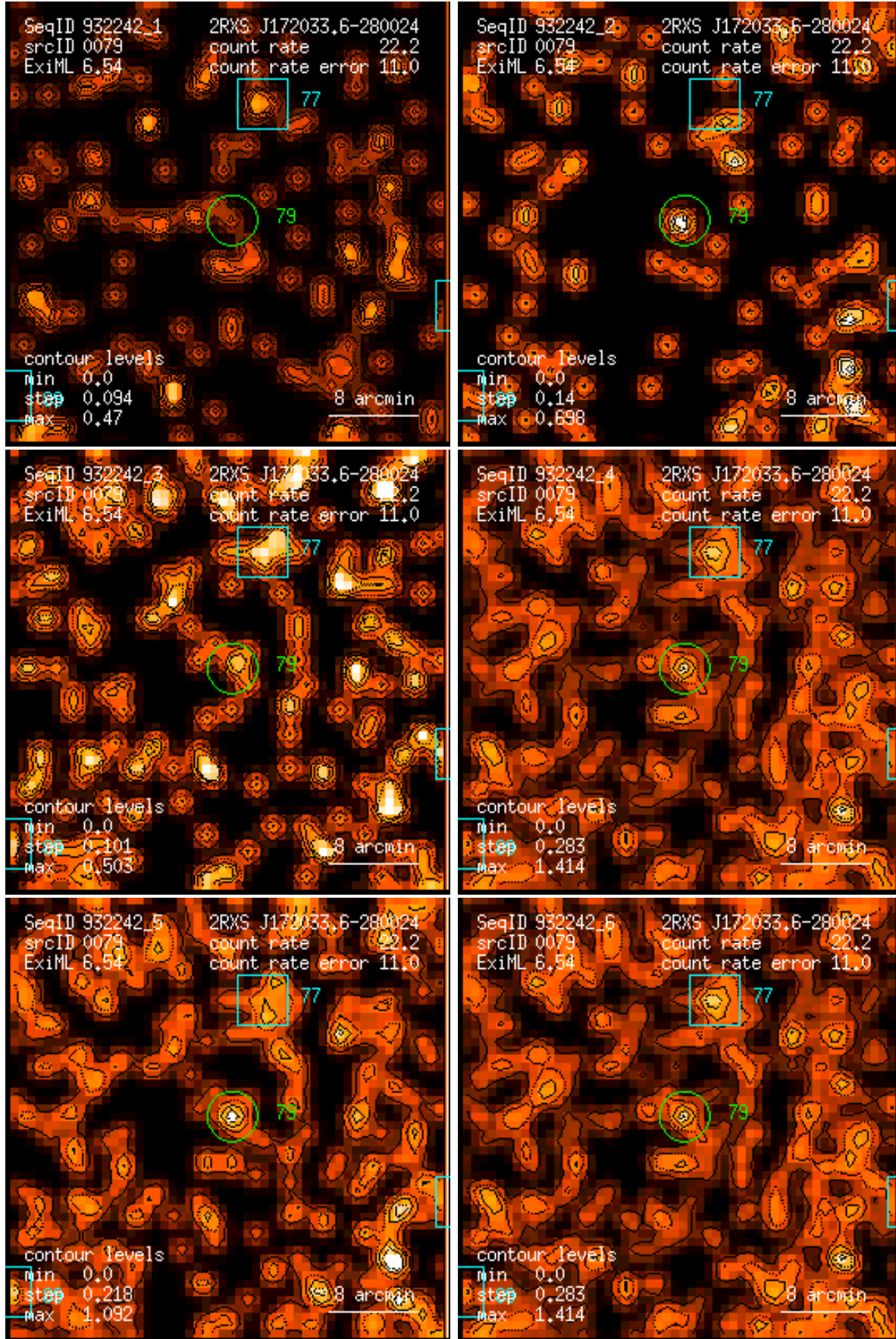
Figure 79: RASS 932242: detection 0079: band rate images, Gaussian filter: (1) PSPC channels 11 – 41, (2) 52 – 90, (3) 91 – 201, (4) 11 – 235, (5) 52 – 201, (6) 11 – 201. Broad band rates in counts/ks. Band rate contour levels in counts/ks/arcmin 2 .
