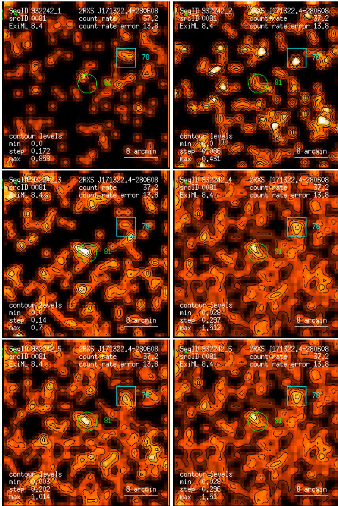
Figure 81: RASS 932242: detection 0081: band rate images, Gaussian filter: (1) PSPC channels 11 – 41, (2) 52 – 90, (3) 91 – 201, (4) 11 – 235, (5) 52 – 201, (6) 11 – 201. Broad band rates in counts/ks. Band rate contour levels in counts/ks/arcmin 2 .
