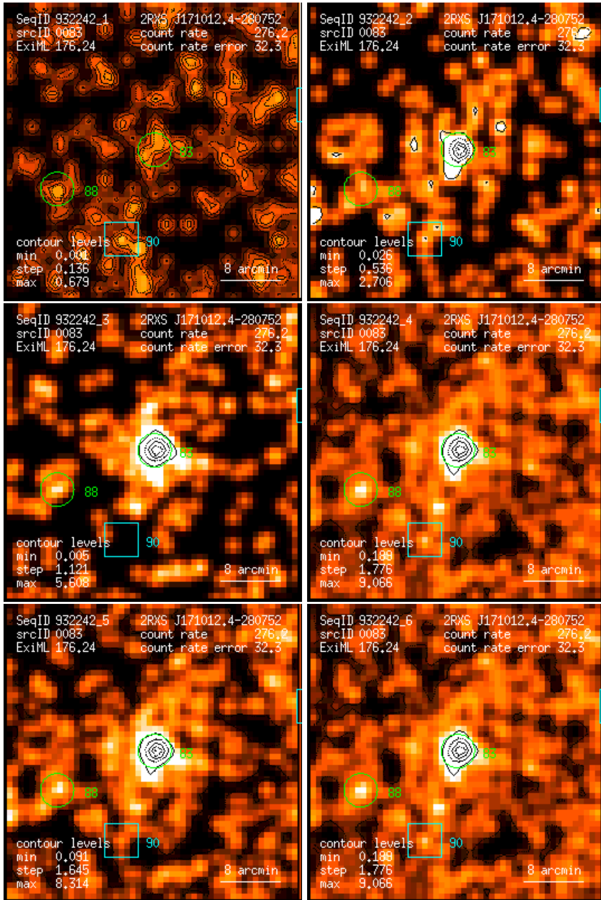
Figure 83: RASS 932242: detection 0083: band rate images, Gaussian filter: (1) PSPC channels 11 – 41, (2) 52 – 90, (3) 91 – 201, (4) 11 – 235, (5) 52 – 201, (6) 11 – 201. Broad band rates in counts/ks. Band rate contour levels in counts/ks/arcmin 2 .
