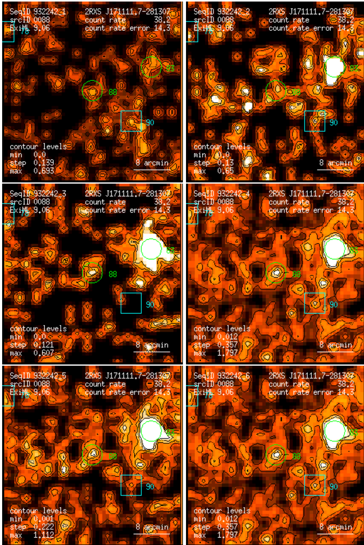
Figure 88: RASS 932242: detection 0088: band rate images, Gaussian filter: (1) PSPC channels 11 – 41, (2) 52 – 90, (3) 91 – 201, (4) 11 – 235, (5) 52 – 201, (6) 11 – 201. Broad band rates in counts/ks. Band rate contour levels in counts/ks/arcmin 2 .
