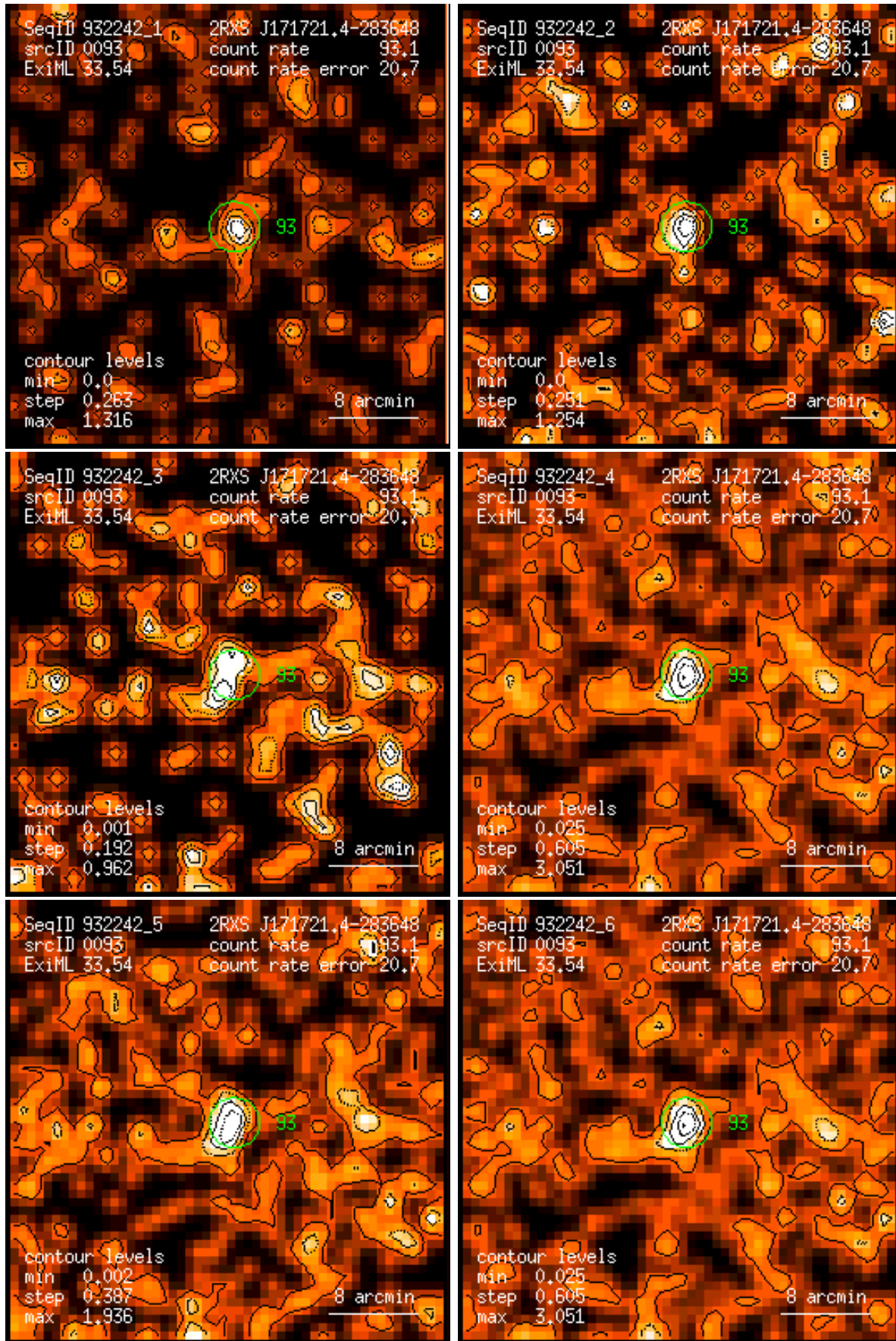
Figure 93: RASS 932242: detection 0093: band rate images, Gaussian filter: (1) PSPC channels 11 – 41, (2) 52 – 90, (3) 91 – 201, (4) 11 – 235, (5) 52 – 201, (6) 11 – 201. Broad band rates in counts/ks. Band rate contour levels in counts/ks/arcmin 2 .
