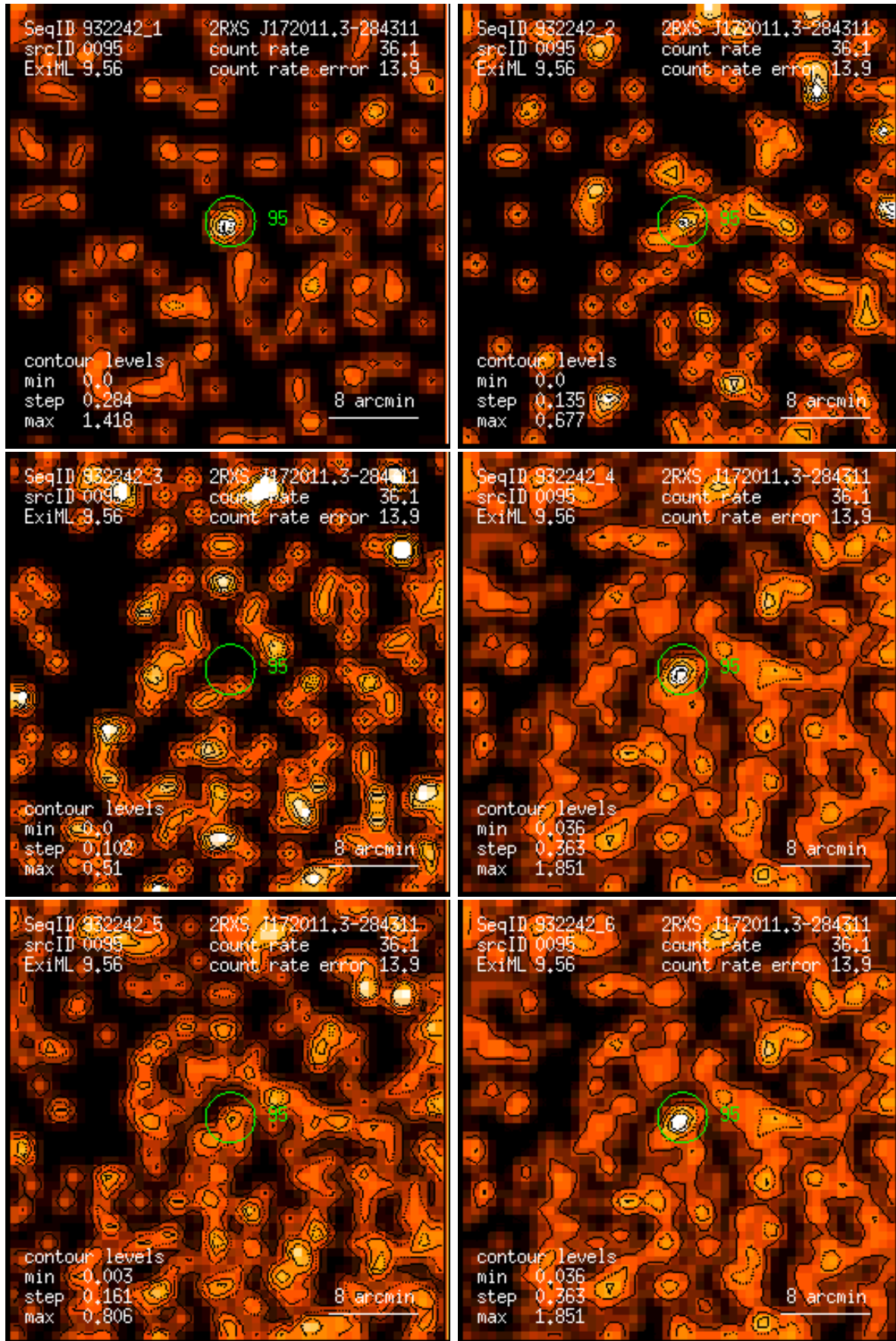
Figure 95: RASS 932242: detection 0095: band rate images, Gaussian filter: (1) PSPC channels 11 – 41, (2) 52 – 90, (3) 91 – 201, (4) 11 – 235, (5) 52 – 201, (6) 11 – 201. Broad band rates in counts/ks. Band rate contour levels in counts/ks/arcmin 2 .
