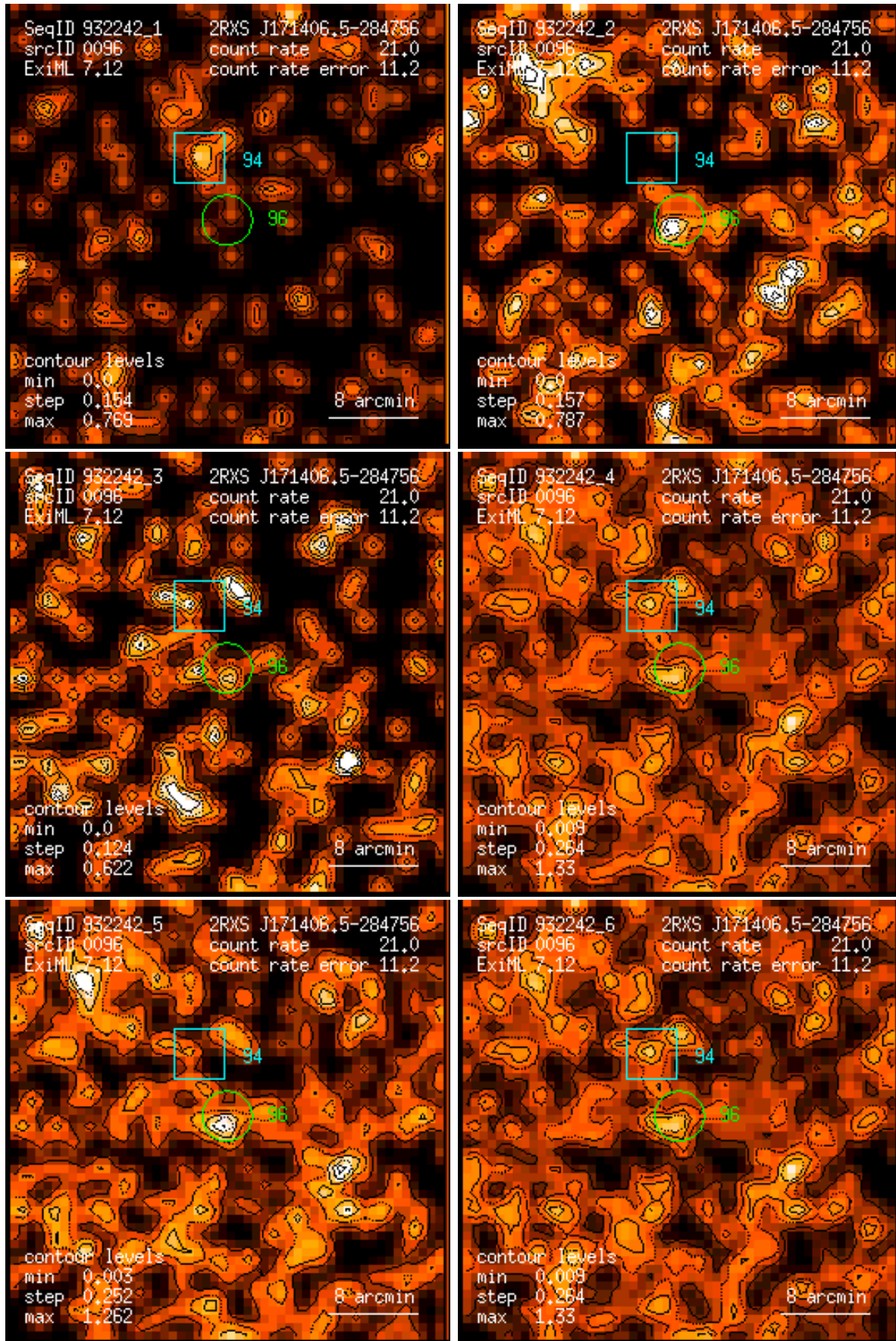
Figure 96: RASS 932242: detection 0096: band rate images, Gaussian filter: (1) PSPC channels 11 – 41, (2) 52 – 90, (3) 91 – 201, (4) 11 – 235, (5) 52 – 201, (6) 11 – 201. Broad band rates in counts/ks. Band rate contour levels in counts/ks/arcmin 2 .
