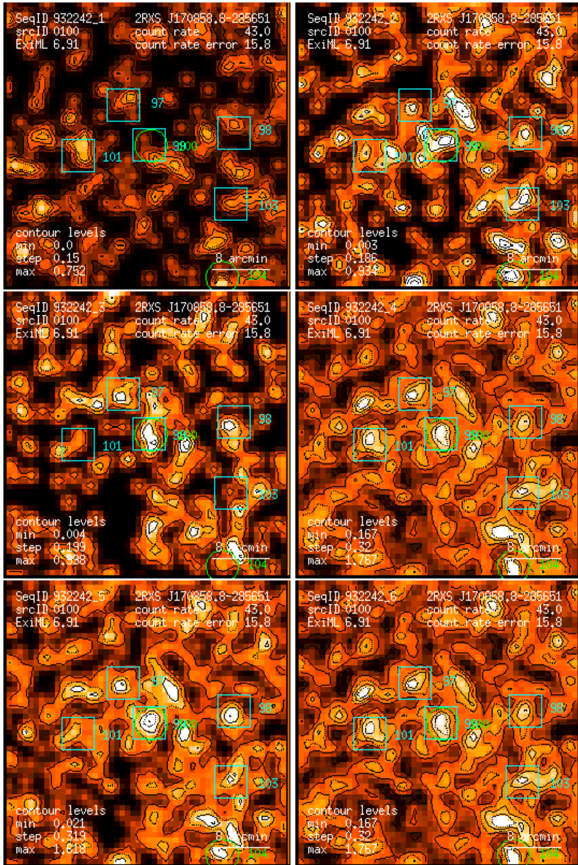
Figure 100: RASS 932242: detection 0100: band rate images, Gaussian filter: (1) PSPC channels 11 – 41, (2) 52 – 90, (3) 91 – 201, (4) 11 – 235, (5) 52 – 201, (6) 11 – 201. Broad band rates in counts/ks. Band rate contour levels in counts/ks/arcmin 2 .
