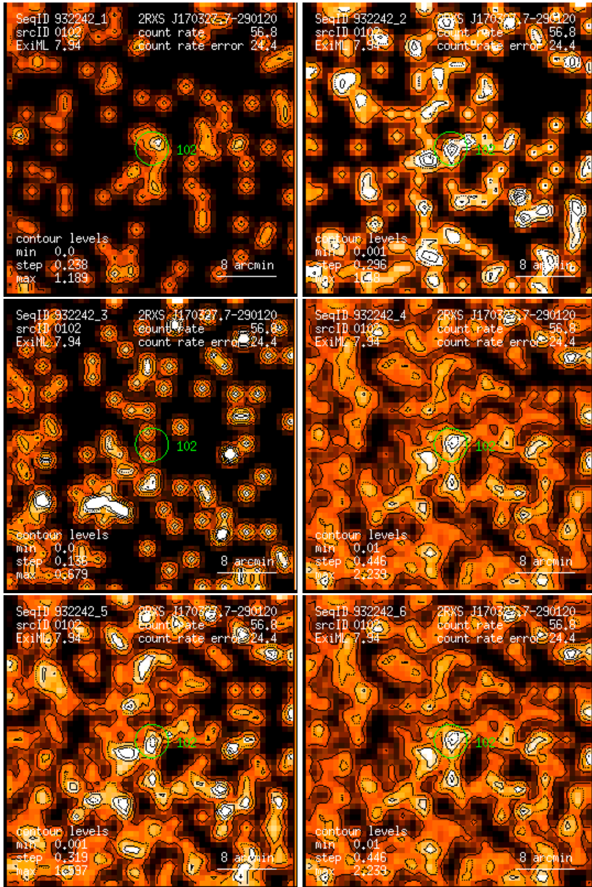
Figure 102: RASS 932242: detection 0102: band rate images, Gaussian filter: (1) PSPC channels 11 – 41, (2) 52 – 90, (3) 91 – 201, (4) 11 – 235, (5) 52 – 201, (6) 11 – 201. Broad band rates in counts/ks. Band rate contour levels in counts/ks/arcmin 2 .
