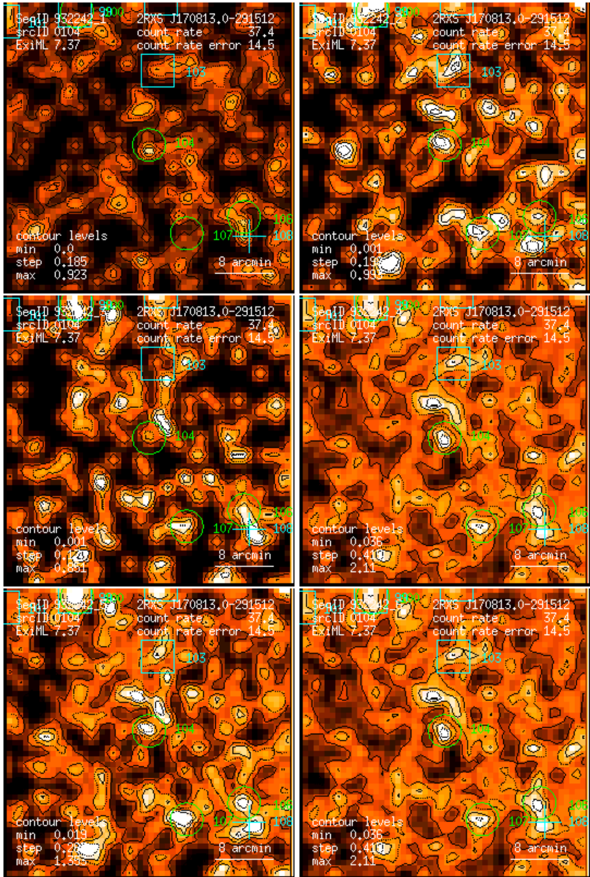
Figure 104: RASS 932242: detection 0104: band rate images, Gaussian filter: (1) PSPC channels 11 – 41, (2) 52 – 90, (3) 91 – 201, (4) 11 – 235, (5) 52 – 201, (6) 11 – 201. Broad band rates in counts/ks. Band rate contour levels in counts/ks/arcmin 2 .
