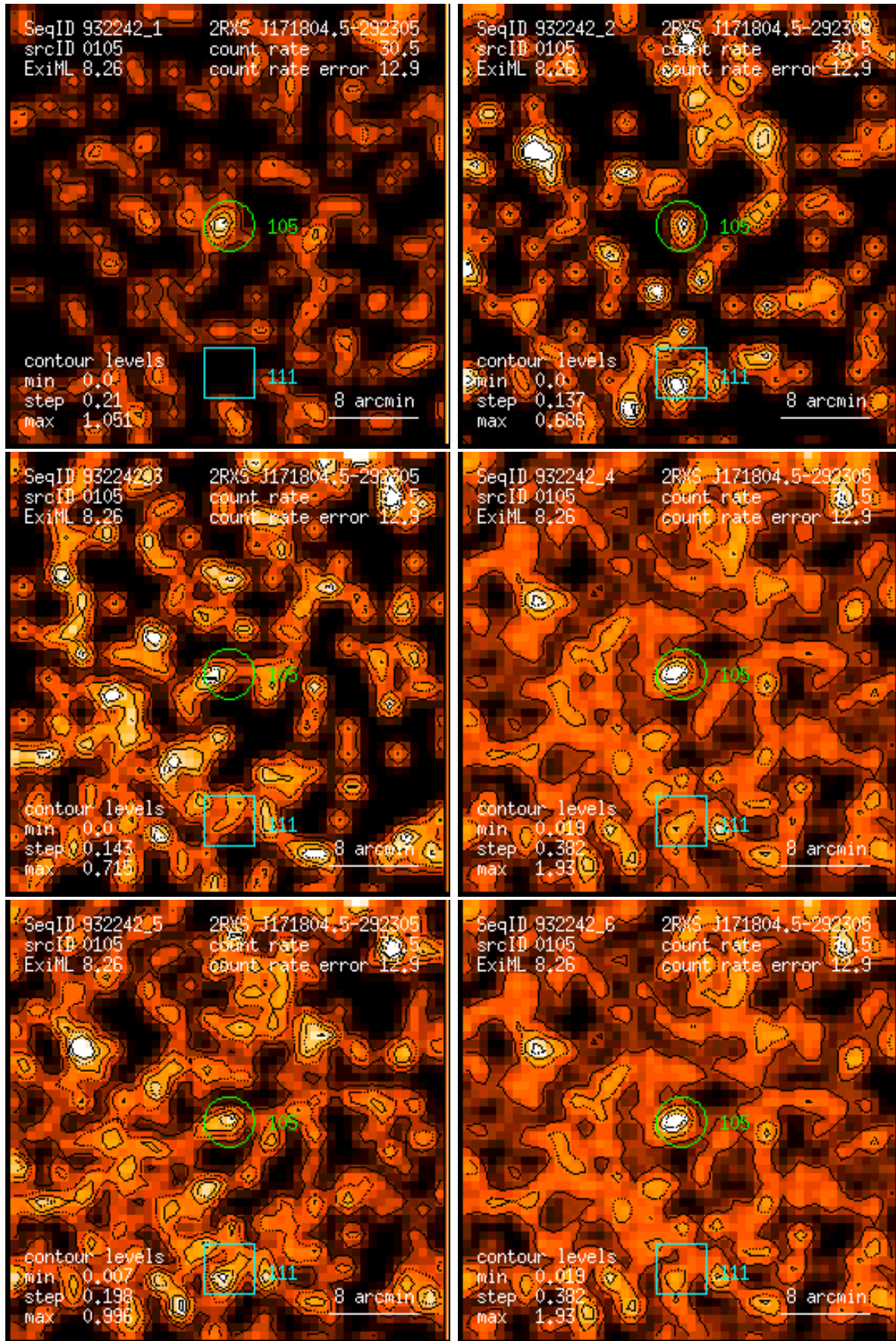
Figure 105: RASS 932242: detection 0105: band rate images, Gaussian filter: (1) PSPC channels 11 – 41, (2) 52 – 90, (3) 91 – 201, (4) 11 – 235, (5) 52 – 201, (6) 11 – 201. Broad band rates in counts/ks. Band rate contour levels in counts/ks/arcmin 2 .
