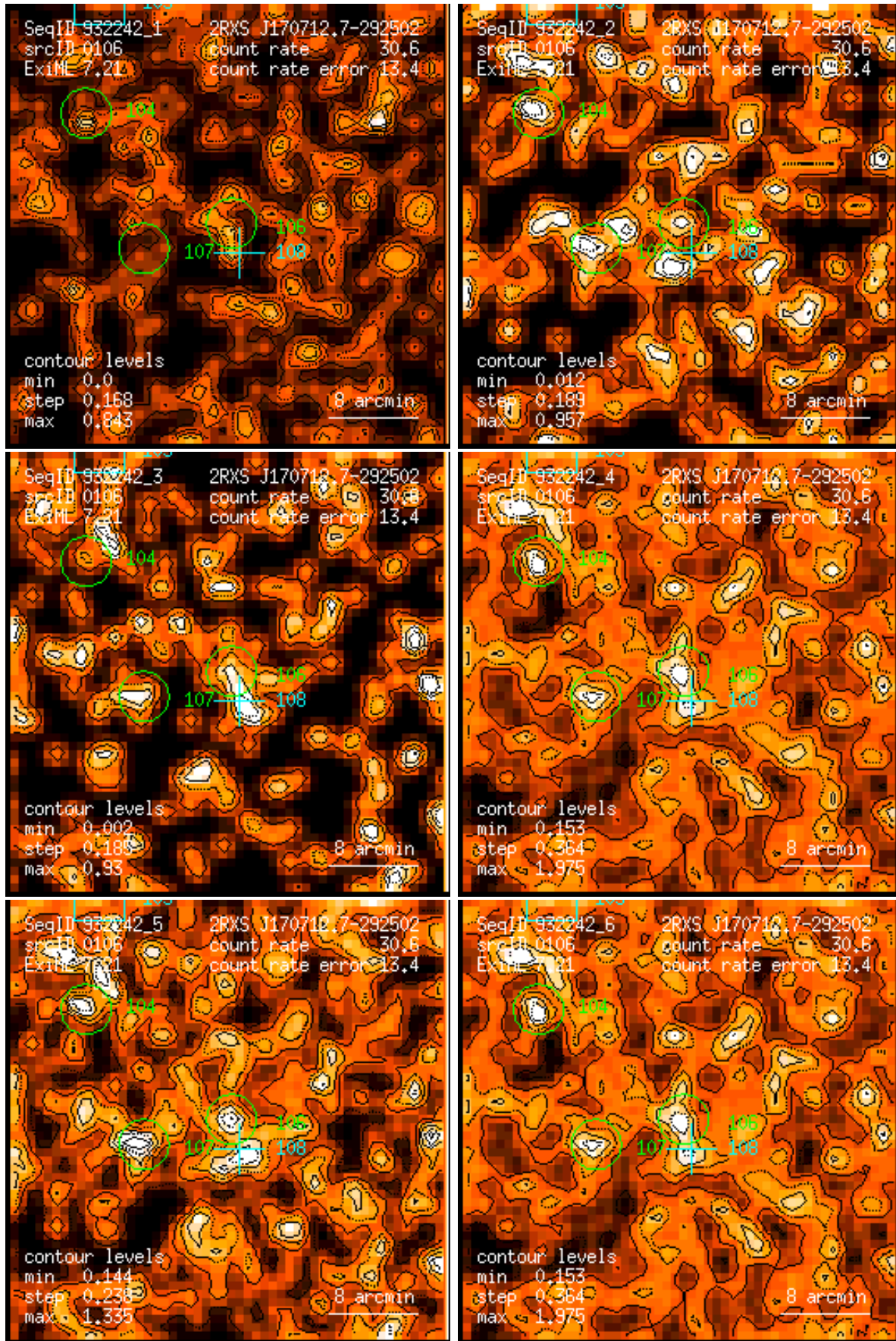
Figure 106: RASS 932242: detection 0106: band rate images, Gaussian filter: (1) PSPC channels 11 – 41, (2) 52 – 90, (3) 91 – 201, (4) 11 – 235, (5) 52 – 201, (6) 11 – 201. Broad band rates in counts/ks. Band rate contour levels in counts/ks/arcmin 2 .
