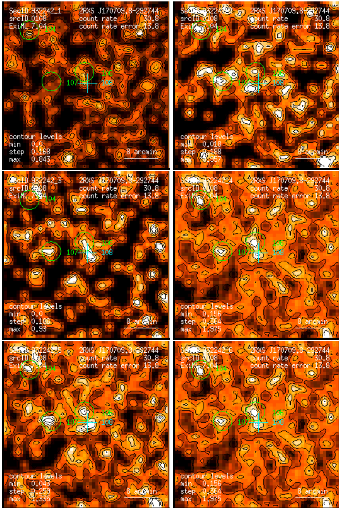
Figure 108: RASS 932242: detection 0108: band rate images, Gaussian filter: (1) PSPC channels 11 – 41, (2) 52 – 90, (3) 91 – 201, (4) 11 – 235, (5) 52 – 201, (6) 11 – 201. Broad band rates in counts/ks. Band rate contour levels in counts/ks/arcmin 2 .
