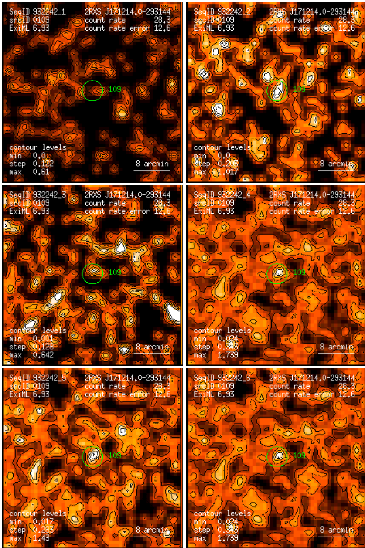
Figure 109: RASS 932242: detection 0109: band rate images, Gaussian filter: (1) PSPC channels 11 – 41, (2) 52 – 90, (3) 91 – 201, (4) 11 – 235, (5) 52 – 201, (6) 11 – 201. Broad band rates in counts/ks. Band rate contour levels in counts/ks/arcmin 2 .
