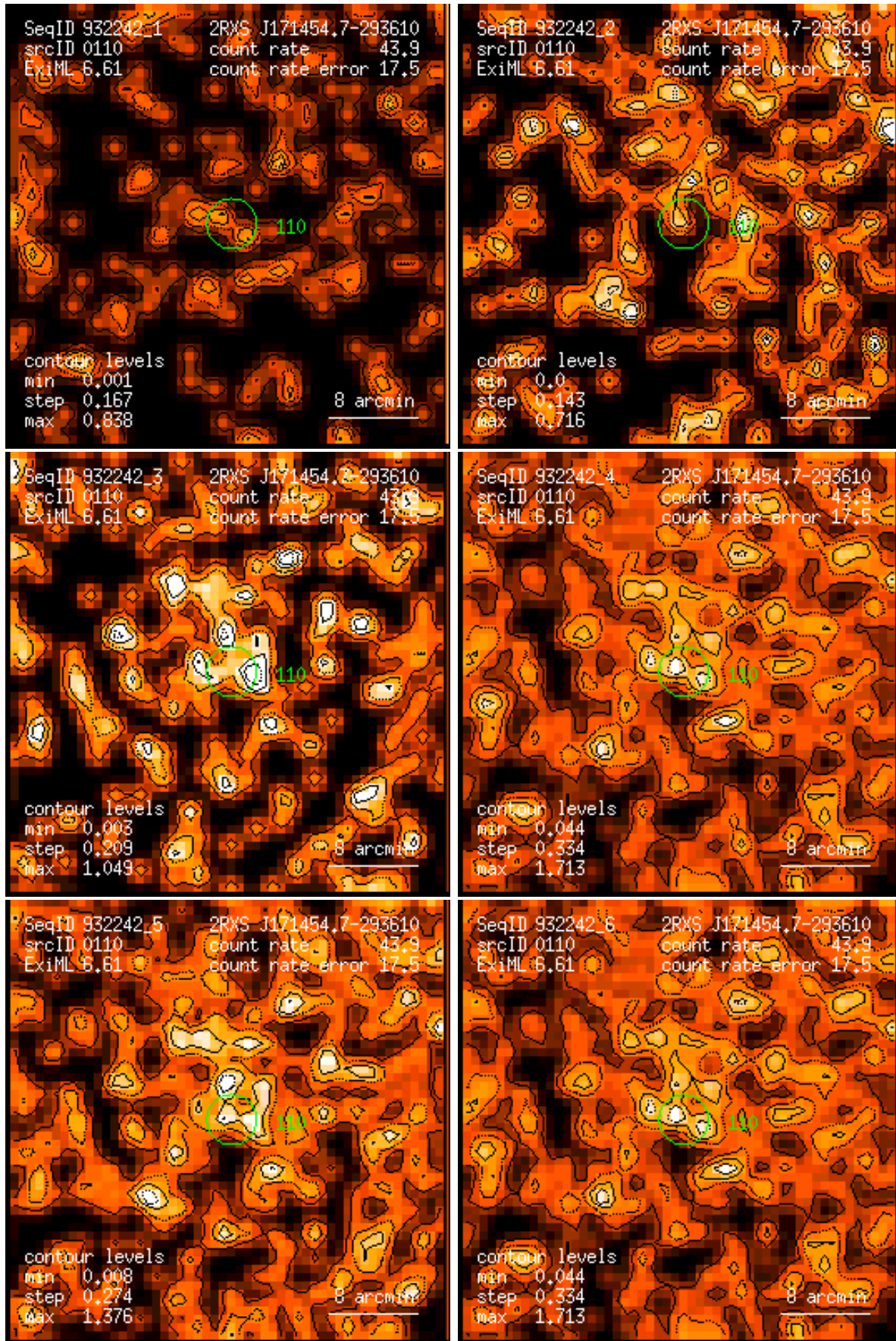
Figure 110: RASS 932242: detection 0110: band rate images, Gaussian filter: (1) PSPC channels 11 – 41, (2) 52 – 90, (3) 91 – 201, (4) 11 – 235, (5) 52 – 201, (6) 11 – 201. Broad band rates in counts/ks. Band rate contour levels in counts/ks/arcmin 2 .
