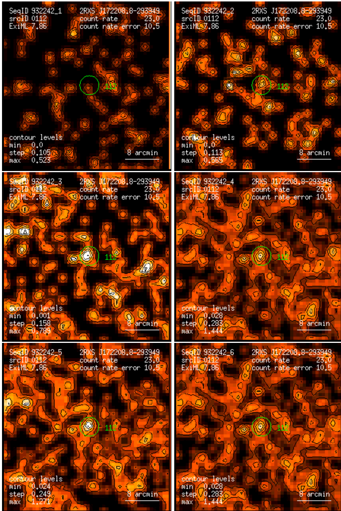
Figure 112: RASS 932242: detection 0112: band rate images, Gaussian filter: (1) PSPC channels 11 – 41, (2) 52 – 90, (3) 91 – 201, (4) 11 – 235, (5) 52 – 201, (6) 11 – 201. Broad band rates in counts/ks. Band rate contour levels in counts/ks/arcmin 2 .
