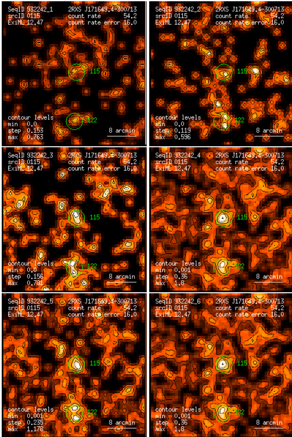
Figure 115: RASS 932242: detection 0115: band rate images, Gaussian filter: (1) PSPC channels 11 – 41, (2) 52 – 90, (3) 91 – 201, (4) 11 – 235, (5) 52 – 201, (6) 11 – 201. Broad band rates in counts/ks. Band rate contour levels in counts/ks/arcmin 2 .
