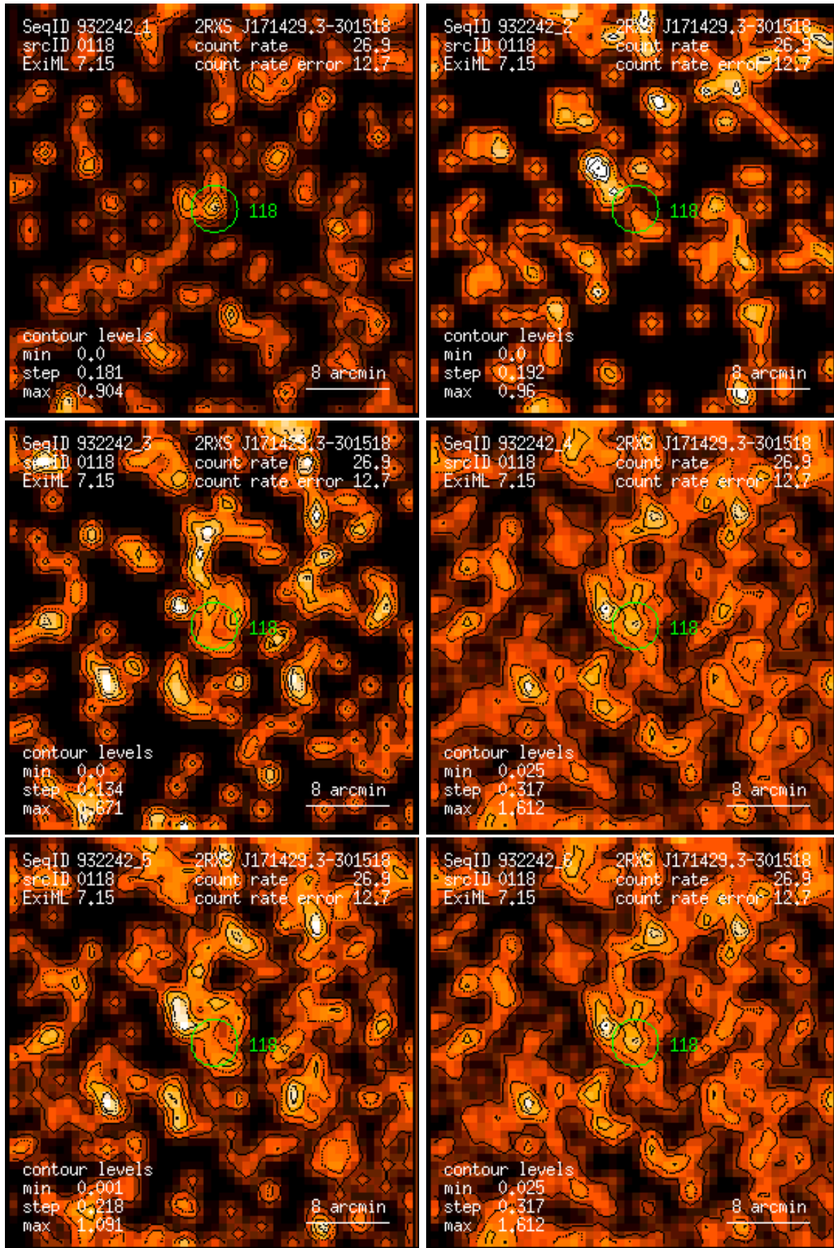
Figure 118: RASS 932242: detection 0118: band rate images, Gaussian filter: (1) PSPC channels 11 – 41, (2) 52 – 90, (3) 91 – 201, (4) 11 – 235, (5) 52 – 201, (6) 11 – 201. Broad band rates in counts/ks. Band rate contour levels in counts/ks/arcmin 2 .
