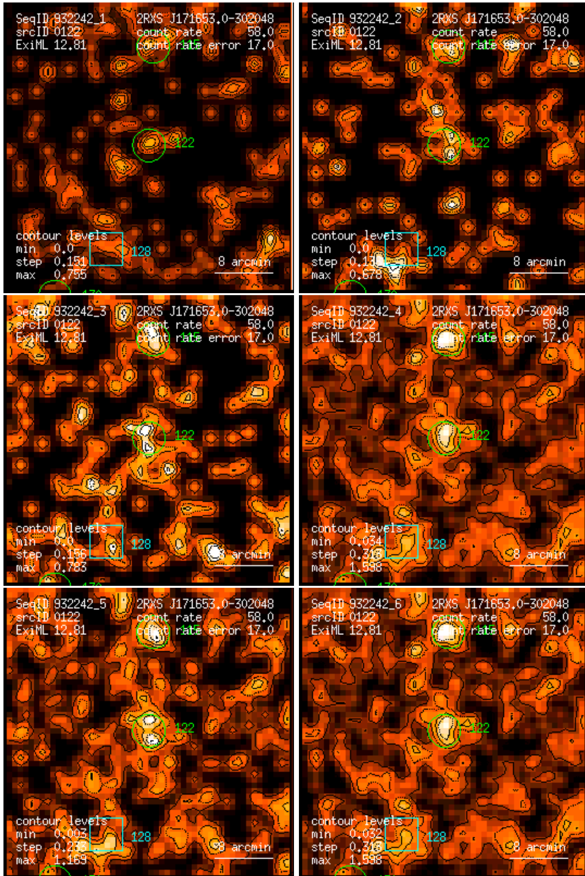
Figure 122: RASS 932242: detection 0122: band rate images, Gaussian filter: (1) PSPC channels 11 – 41, (2) 52 – 90, (3) 91 – 201, (4) 11 – 235, (5) 52 – 201, (6) 11 – 201. Broad band rates in counts/ks. Band rate contour levels in counts/ks/arcmin 2 .
