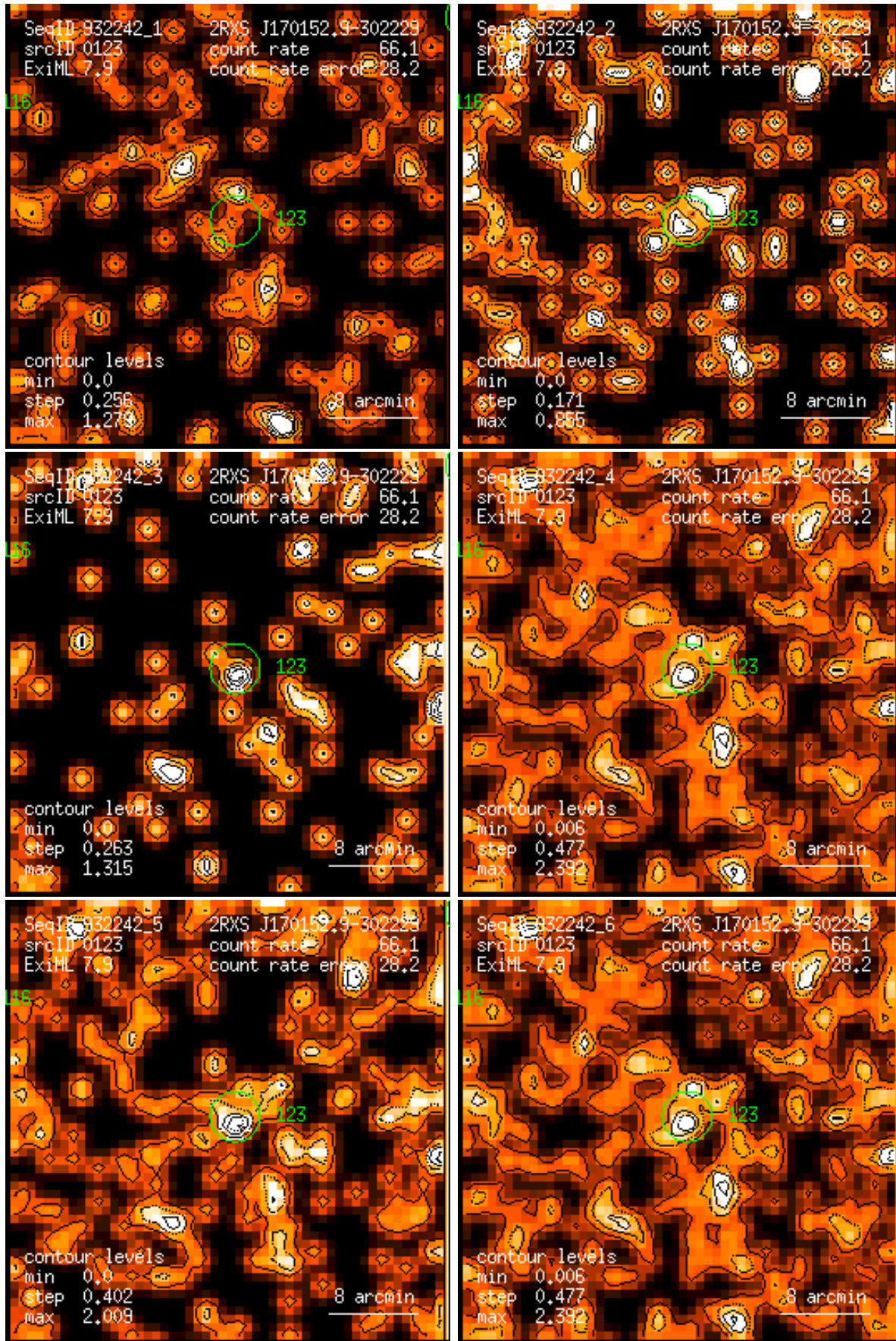
Figure 123: RASS 932242: detection 0123: band rate images, Gaussian filter: (1) PSPC channels 11 – 41, (2) 52 – 90, (3) 91 – 201, (4) 11 – 235, (5) 52 – 201, (6) 11 – 201. Broad band rates in counts/ks. Band rate contour levels in counts/ks/arcmin 2 .
